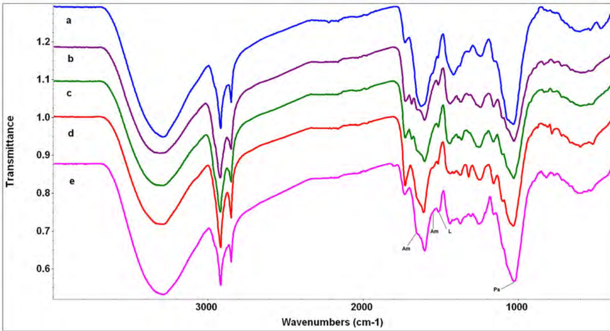
Figure 1. FTIR spectra of gypsogag species. The scale of the Y axis is offset for illustration purposes. a) Linum suffruticosum (blue), b) Rosmarinus officinalis (purple), c) Salvia lavandulifolia (green), d) Teucrium polium subsp. capitatum (red), e) Thymelaea tinctoria (pink). Abbreviations of compound peaks: Am: Amide, L: Lignin/Phenolic backbone, Ps: Polysaccharides. doi:10.1371/journal.pone.0107285.g001
