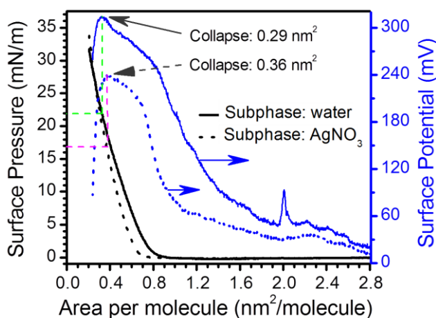
Figure 2. Representative surface pressure and surface potential vs. area per molecule isotherms formed from \mathbf{1H}_2 on pure water ( \mathbf{1H}_2 ) and 4\cdot 10^{-4} \text{ M} \text{AgNO}_3 ( \mathbf{1HAg}^+ ) aqueous sub-phases.
