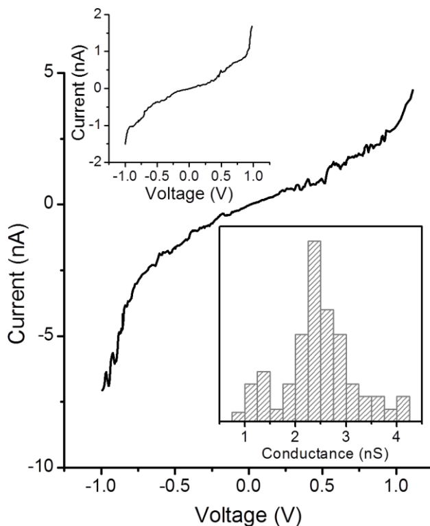
Figure 8. Representative I - V curve obtained by positioning the c-AFM tip on top of AgNPs in a 1AgNP film. The set-point force used was 17.5 nN. Inset bottom: conductance histogram built from all the experimental data from -0.5 to 0.5 V for each I - V curve recorded (ca. 250 curves) at this set-point force. Inset top: representative I - V curve obtained by positioning the c-AFM tip on the organic monolayer not covered by AgNPs when a set-point force of 8 nN was applied; at higher set-point forces the LB film is damaged.
