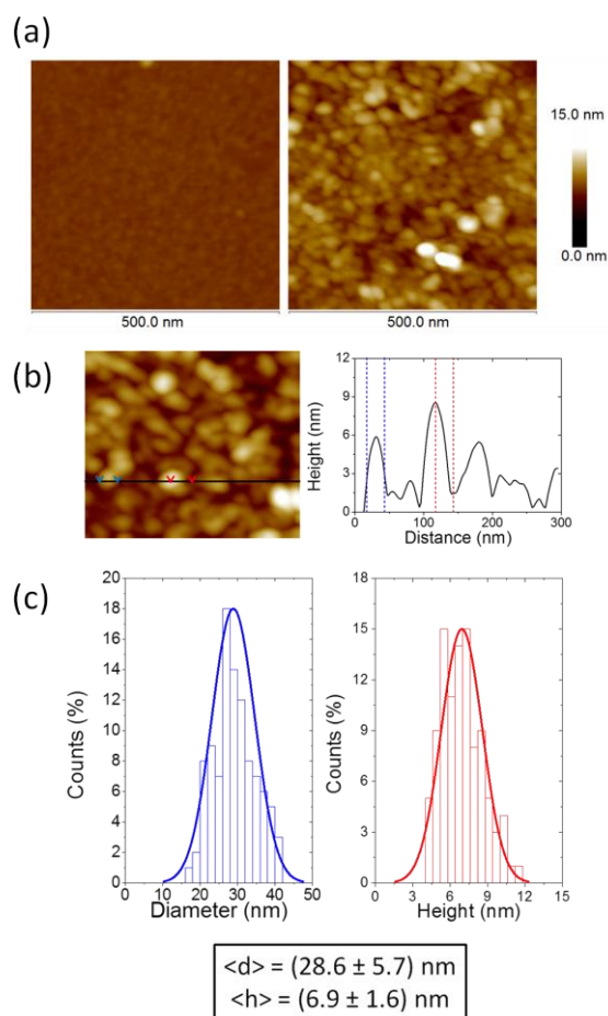
Figure 6. (a) 500 \times 500 \text{ nm}^2 AFM images of a monolayer LB film of 1\text{Ag}^+ transferred from an \text{AgNO}_3 aqueous solution before (left panel) and after irradiation for 15 minutes at
