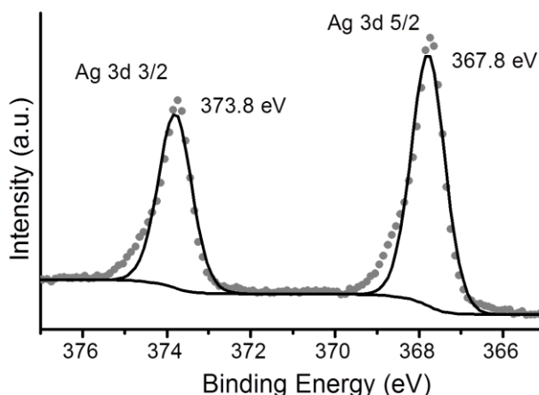
Figure 5. XPS spectra of Ag(3d) photoelectrons of a one-layer LB film of 1\text{AgNP} , formed following transference of a LB film of 1\text{Ag}^+ from an \text{AgNO}_3 aqueous solution and irradiated at 254 nm for 15 minutes.
