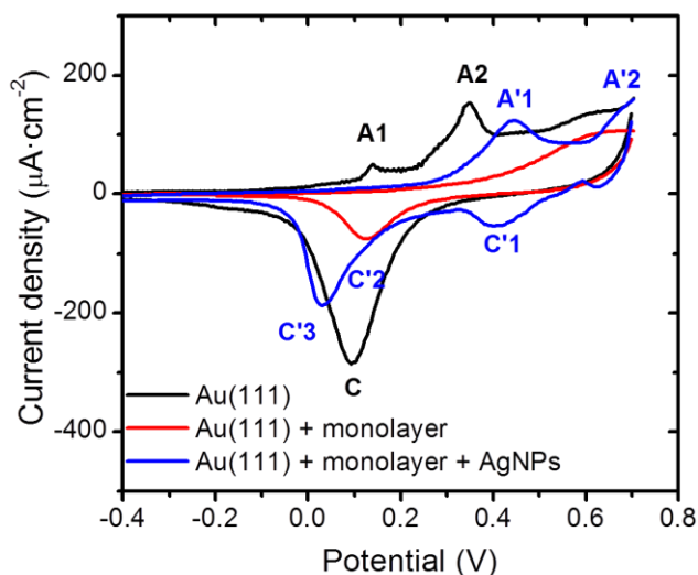
Figure 9. Black: cyclic voltammograms recorded for a bare Au(111) electrode. Red: monolayer of 1H 2 transferred onto a Au(111) substrate. Blue: Au(111)/monolayer with overlying silver nanoparticles ( 1AgNP ). All the voltammograms were recorded in a 0.1 M NaOH aqueous solution at 0.1 V·s -1 using a Ag/AgCl, KCl (3M) reference electrode.
