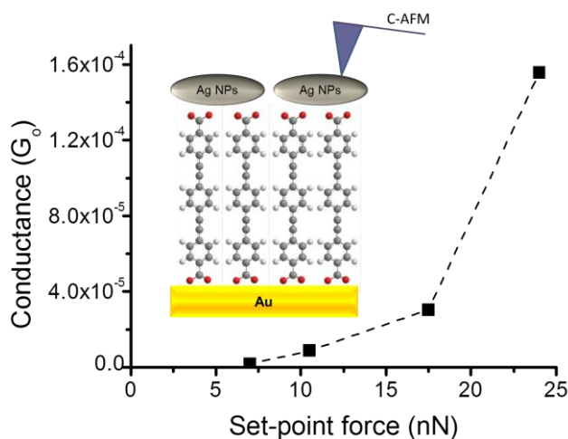
Figure 7. Average conductance values measured by locating the tip of the c-AFM on top of AgNPs at the indicated set-point forces. Inset: a scheme of the studied metal|1AgNPs structures.
