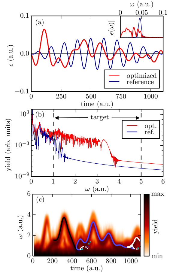
FIG. 2. (Color online) Same as Fig. 1 but for an extended target range (up to \omega = 5 a.u.) and for the gradient-based BFGS optimization algorithm. In (c), energies of an electron calculated from the semiclassical model upon its first, second, third, and fourth return to the origin are shown with black, blue (medium gray), white, and cyan (light gray) curves, respectively.
