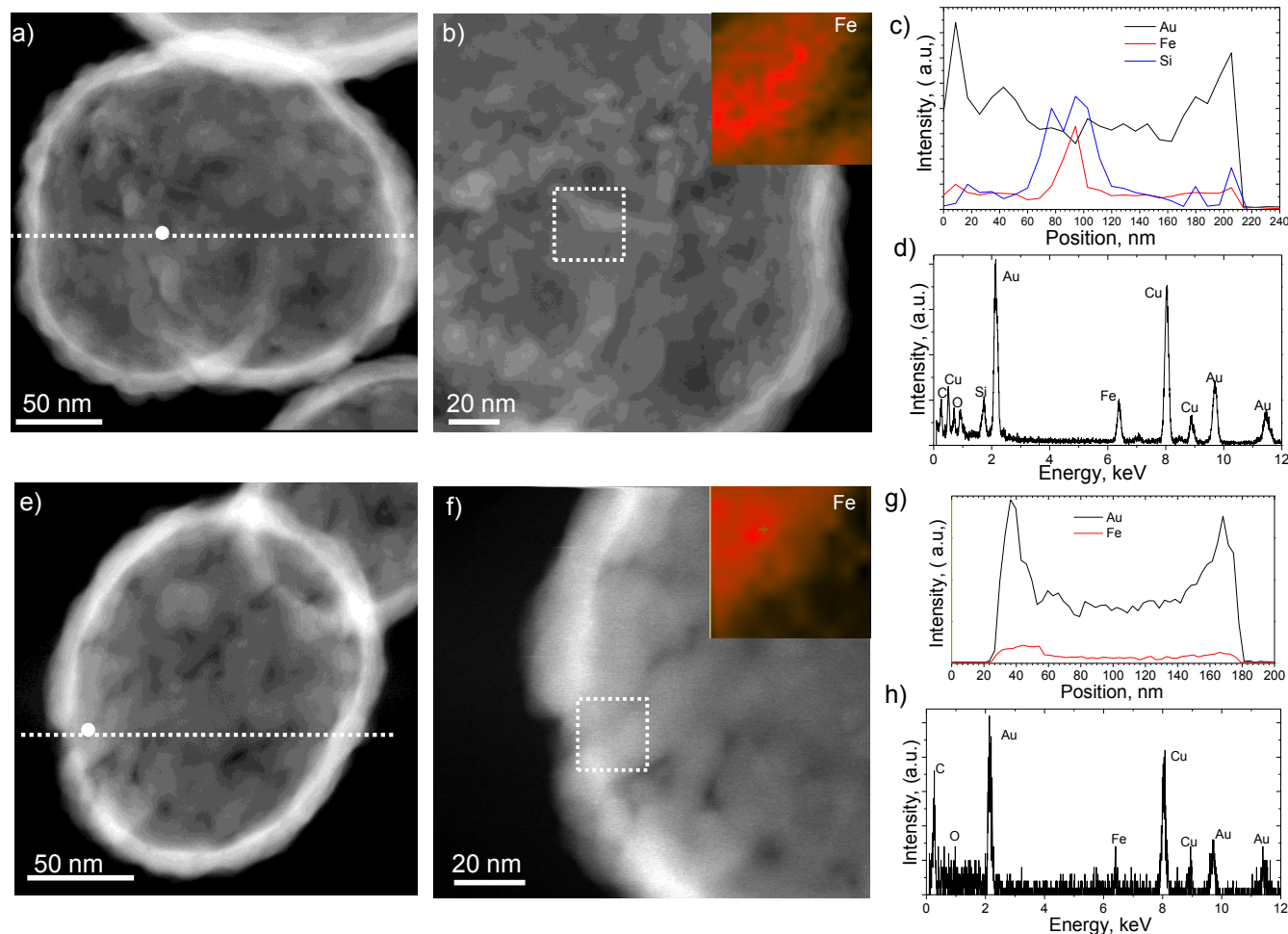
Figure 4.- Characterization of partially hollow (PH) and hollow (H) gold-magnetic nanoparticles after \text{SiO}_2 etching by BHF and NaOH approaches. BHF etching: a) STEM-HAADF image of a PH gold-magnetic nanoparticle obtained after 2 hours with a 0,001 volume of BHF/volume ratio of nanoshell dispersion. b) STEM-HAADF image of a detail area where a SPION is located under the Au shell. Inset is an Fe elemental mapping from the selected area in figure 4-b. c) Au, Si and Fe EDS profile along the selected line in figure 4-a. Highest Fe and Si signal were detected in a location shifted from the NP center. d) EDS spectra at the point selected in figure 4-a. The Si peak indicates that there is a silicon oxide layer protecting the SPION core. NaOH etching: e) STEM-HAADF image of a hollow gold-magnetic nanoparticle obtained after 15 minutes etching with a 1 volume of NaOH(3M)/volume of nanoshell dispersion. f) STEM-HAADF image of a detail area where a \text{SiO}_2 -SPION core-shell nanoparticle is located under the Au shell. Inset is an Fe elemental mapping from the selected area in figure 4-f. g) Au and Fe EDS profile along the selected line in figure 4-e. Fe was detected close to the gold shell. Si was not detected h) EDS spectra at the point selected in figure 4-e.
