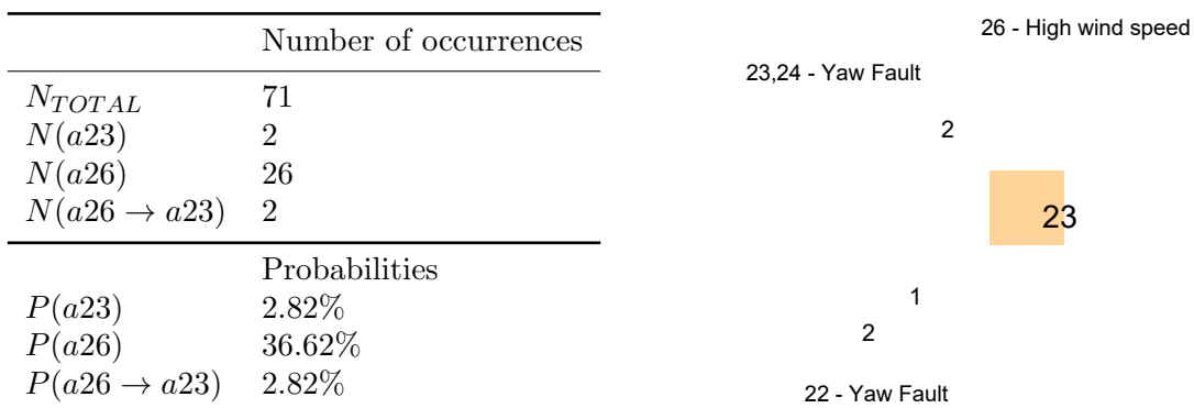
Figure 8. Alarm statistics and Venn diagram before a failure of the yaw system
