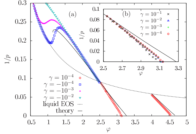
FIG. 3. (Color online) (a) Compressions ( \gamma > 0 ) and decompressions ( \gamma < 0 ) of an initial equilibrium state at \varphi_0 = 2.5 and 4.0 . The results are averaged over N_s = 100 samples. The theoretical curves uses data from Ref. [17] and from this work [36]. (b) Compression data are indistinguishable for \gamma \leq 0.01 .
