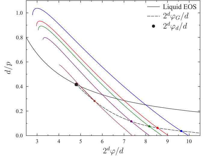
FIG. 1. (Color online) Phase diagram of the HS and MK models in the limit d \rightarrow \infty . Results are partially derived from Ref. [17], complemented by results obtained for the Gardner phase [36]. The liquid equation of state (EOS) given by Eq. (6) (full black line) gives p/d = (2^d \phi/d)/2 in the limit d \rightarrow \infty . The black dot denotes the dynamical glass transition at 2^d \phi_d/d = 4.8 . Glass EOSs from state following (SF) for 2^d \phi_0/d = 5, 6, 6.667, 7, 8 are also reported (thin colored lines, from left to right). The envelope for the Gardner transition for each SF (colored dot) is given by the dashed line.
