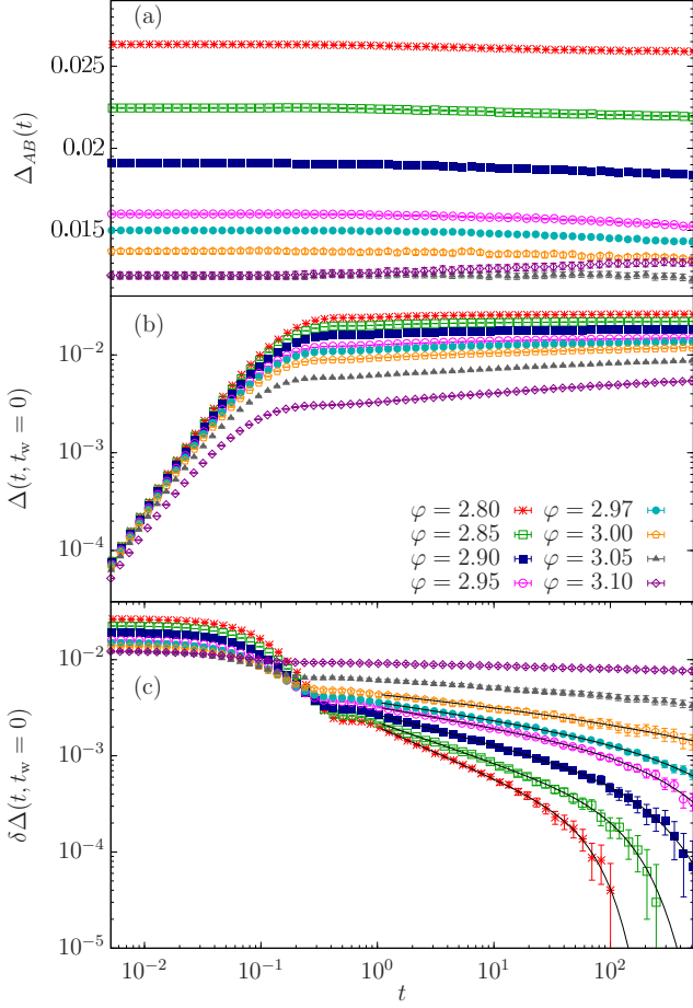
FIG. 4. (Color online) SF from \varphi_0 = 2.50 gives (a) \Delta_{AB}(t) , (b) \Delta(t, t_w = 0) , and (c) \delta\Delta(t, t_w = 0) at different \varphi . Solid lines are fits to Eq. (21) (bottom panel).
