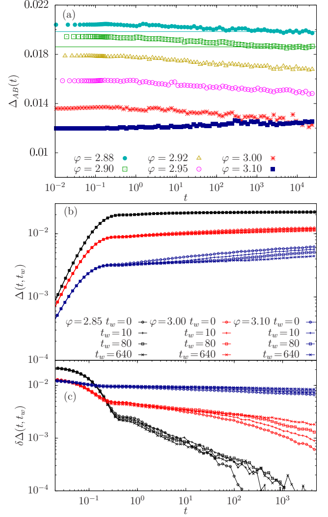
FIG. 5. (Color online) (a) Long-time results for \Delta_{AB}(t) . The data show that, for \varphi < \varphi_G , \Delta_{AB}(t) saturates at its asymptotic value (dotted line) in the long-time limit (see, e.g., \varphi = 2.88, 2.90 ). Panels (b) \Delta(t, t_w) and (c) \delta\Delta(t, t_w) are plotted as a function of t for various \varphi and t_w .
