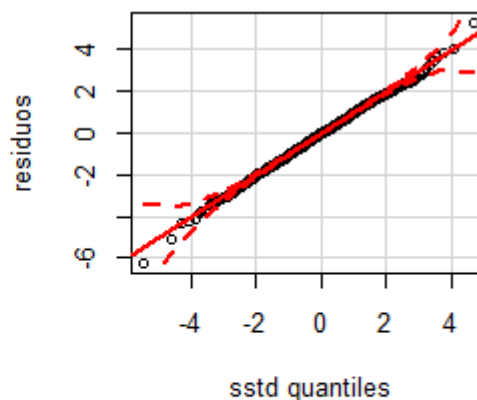
ARMA (0,0)-GARCH (4,1)
