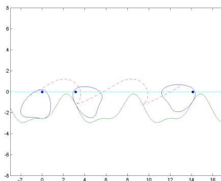
Figura 1.15: Caso y(x) = -1,887365 - \frac{2 \cos(x)}{3} + \sin(x) - \frac{\sin(2x)}{2}
