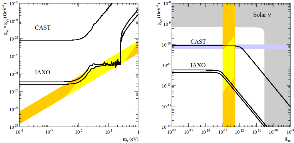
Figure 8.6: Left: IAXO sensitivity line for g_{ae} \times g_{a\gamma} as a function of m_a , assuming a dominating non-hadronic solar axion emission. The orange band is related with the DSFZ model. The yellow band corresponds to those models in which the relation of g_{ae} with m_a is more suitable. The recent limit of CAST [75] is also shown. Right: IAXO sensitivity on g_{ae} and g_{a\gamma} for m_a < 0.01 eV. The gray region is excluded by solar neutrino measurements and the orange band corresponds to values of g_{ae} \sim 1 - 5 \times 10^{-13} . The yellow band represents the more plausible models. The recent limit of CAST [75] is also shown. Helium-burning stars would be perceptibly affected in the blue band, in which the parameters above are excluded. Plots taken from [132].
