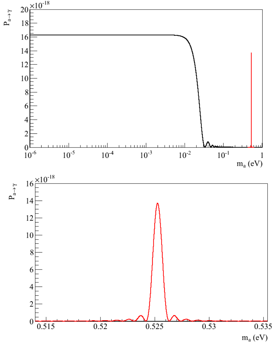
Figure 1.11: Axion to photon probability conversion in function of the axion mass, the calculations are made for axions with an energy of E_a = 4.2 keV, on a transversal magnetic field of B = 8.8 T over a length of L = 9.26 m and with a coupling constant of g_{a\gamma} = 10^{-10} GeV ^{-1} . The black line represent the vacuum case, while the red line assumes ^3\text{He} as buffer gas with a density of \rho = 5 \times 10^{-4} g cm ^{-3} which corresponds to a photon mass of m_\gamma = 0.525 keV. The figure on the top is a general view while the figure on the bottom is a zoom of the buffer gas case.
