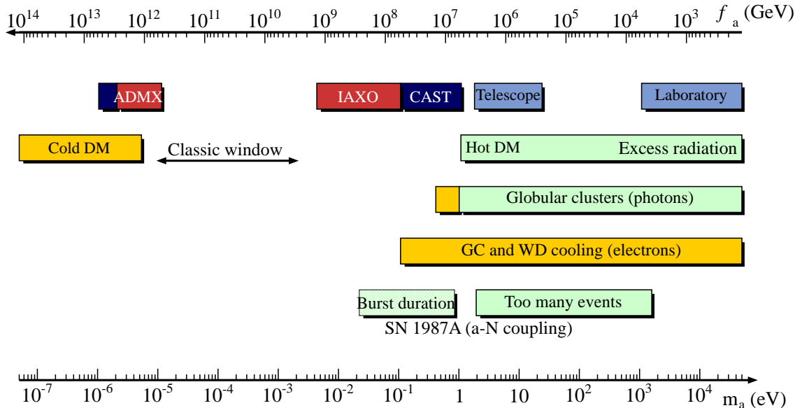
Figure 1.3: Astrophysical and cosmological bounds in combination with experimental searches for axions. Dark blue labels represent experimental search ranges of CAST and ADMX experiments and the red labels correspond to future prospects. Telescope and laboratory searches (light blue labels) are also drawn. Orange labels indicate strong model dependent limits while the green ones are model independent. The limit imposed for the SN 1987A burst has been drawn with a different style due to the uncertainties of the measurements.
