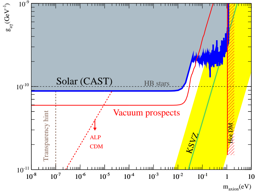
Figure 7.15: Prospects of the expected sensitivity of the new vacuum phase in the CAST experiment (red line), in contrast with the current CAST limit (blue line). ALP hints and theoretical limits presented in chapter 1 are also drawn.
