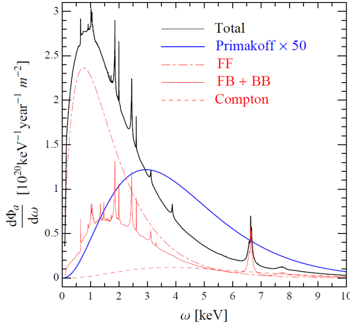
Figure 1.10: Differential solar axion flux at Earth in non-hadronic processes using a coupling constant of g_{ae} = 10^{-13} . Different contributions have been drawn: atomic recombination plus atomic deexcitation (FB + BB), Bremsstrahlung process (FF) and Compton. The solid blue line is the Primakoff emission with g_{a\gamma} = 10^{-12} \text{ GeV}^{-1} which has been multiplied by a factor 50 to make it visible. Plot taken from [60]
