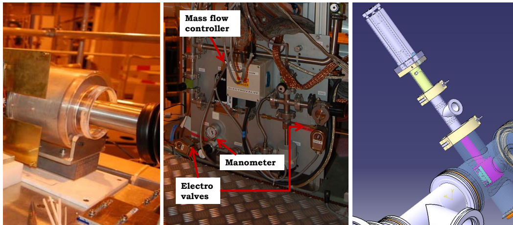
Figure 3.9: Left: Photo of the Sunrise Micromegas shielding. Middle: Photo of the gas panel in which the different parts are labeled. Right: Sketch of the Sunrise manipulator installed on the line during a calibration. For background runs the source is retracted and hidden inside the flange.
