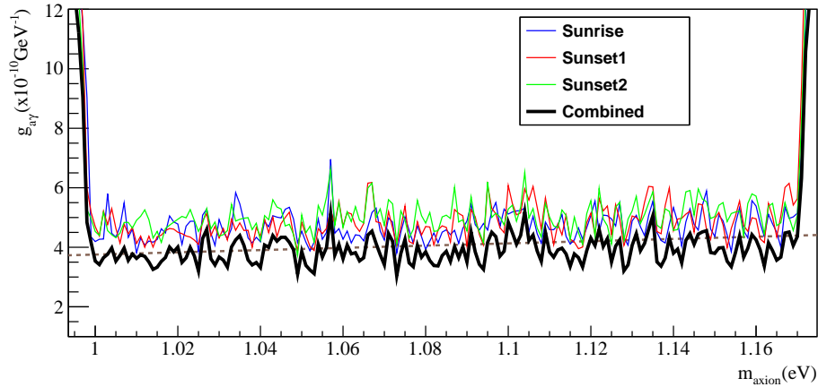
Figure 6.8: Axion to photon coupling upper limit for the different detectors during 2011 data taking campaign. The solid blue line corresponds to the Sunrise detector, the solid red and green lines show the limit for Sunset1 and Sunset2 detectors respectively. The solid black line is the combination of all the detectors and the dashed brown line represents the KSVZ model with E/N = 0 .
