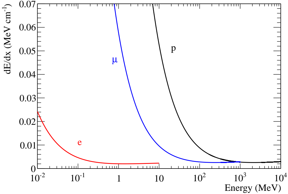
Figure 3.1: Bethe-Bloch parameterization of the stopping power in Ar for different particles: electrons (red), muons (blue) and protons (black). Equation 3.1 has been used for protons and muons while equation 3.2 is used for electrons.
