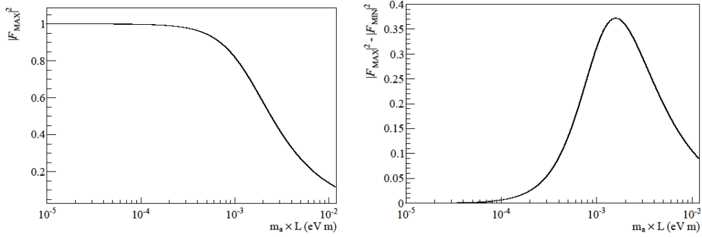
Figure 9.4: Left: Maximum value of |\mathcal{F}_{IS}|^2 versus m_a L , with the cavity oriented perpendicular to the CYGNUS point. Right: Difference of the maximum and minimum values of |\mathcal{F}_{IS}|^2 (with the cavity oriented perpendicular and parallel to the CYGNUS point, respectively) versus m_a L . Plots taken from [139].
