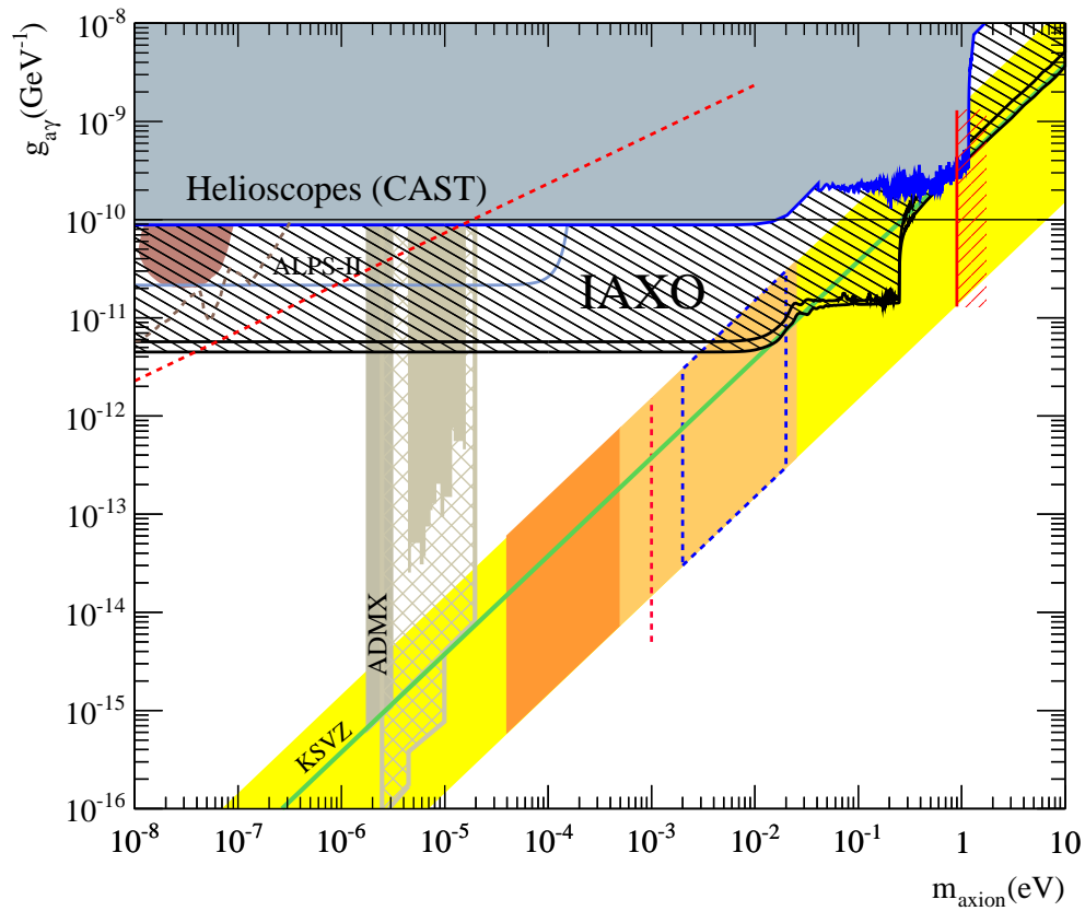
Figure 10.13: Expected sensitivity of IAXO (black filled areas) for hadronic axions, compared with current bounds from CAST and ADMX. Also future prospects of ADMX (dashed brown region) and ALPS-II (light blue line) are shown.
