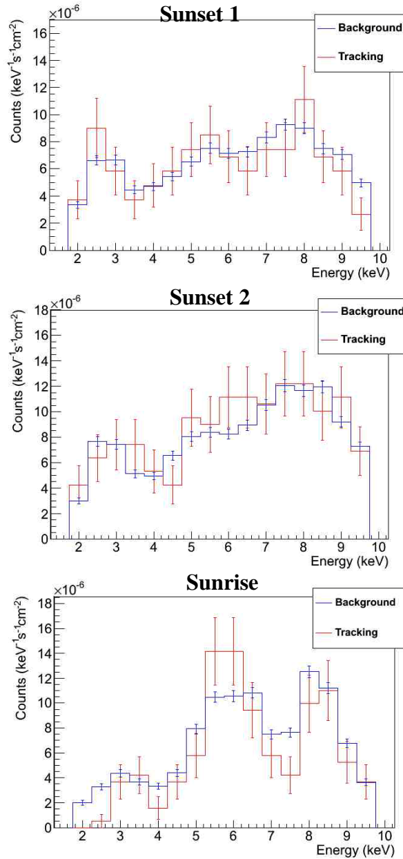
Figure 5.9: Comparison between background (blue bars) and tracking (red bars) spectra during the 2011 data taking campaign. A binning of 0.5 keV has been selected to compute both distributions.
