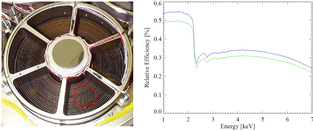
Figure 2.13: Left: Photo of the front view of the ABRIXAS X-ray focusing device. The red circle represents the CAST magnet bore. Right: Efficiency of the telescope as a function of the energy in which two cases are displayed: the 2003 data taking period (blue line) and the following campaigns of data taking (green line). The loss of efficiency is due to the realignment of the telescope during 2004 in order to center the spot in the CCD detector.
