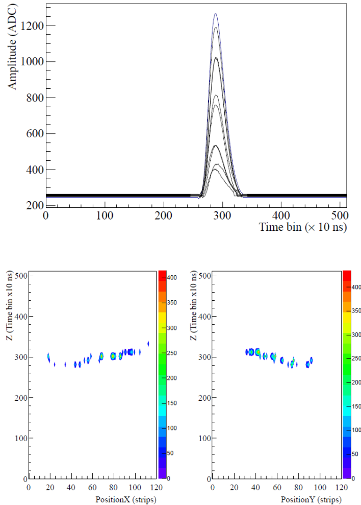
Figure 7.1: Left: Pulses from a 5.9 keV calibration event digitized by the AFTER electronics. Right: The 2D view of a background event acquired with the AFTER electronics in which the two different projections XZ (left) and YZ (right) are shown.
