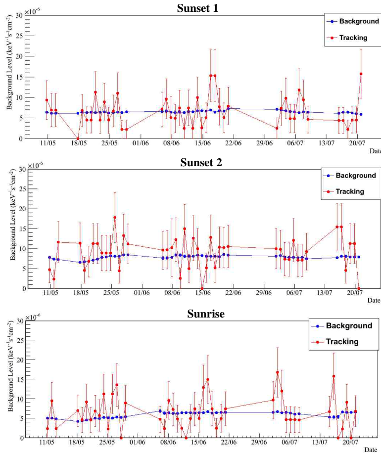
Figure 5.8: Comparison between background (blue dots) and tracking (red dots) levels during the 2011 data taking campaign. The tracking level is computed for single traking while 240 h has been computed to extract the background level. The error bars represent 1 \sigma .
