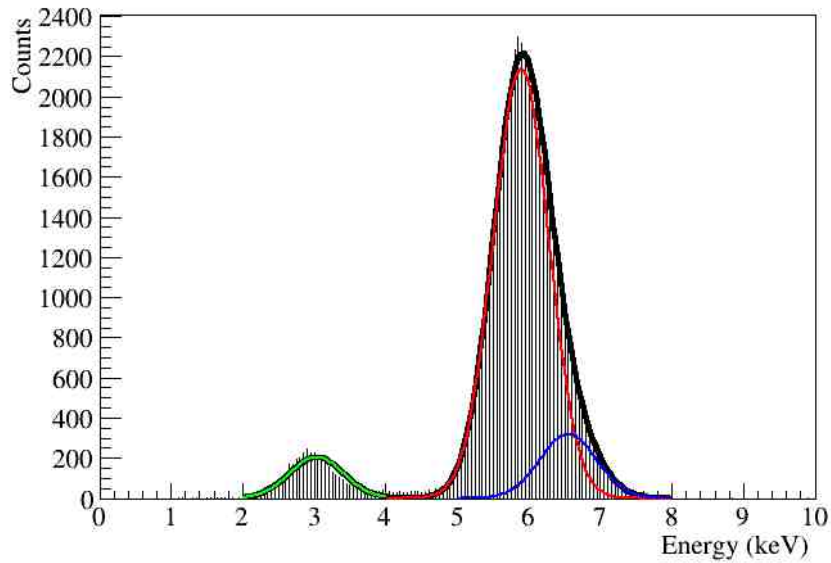
Figure 4.8: ^{55}\text{Fe} spectra in a Micromegas detector in which the three different peaks have been fitted: the escape peak (green line), the 5.9 keV peak (red line) and the 6.5 keV line (blue line). The solid black line is the total fit, computed by the addition of the three Gaussians.
