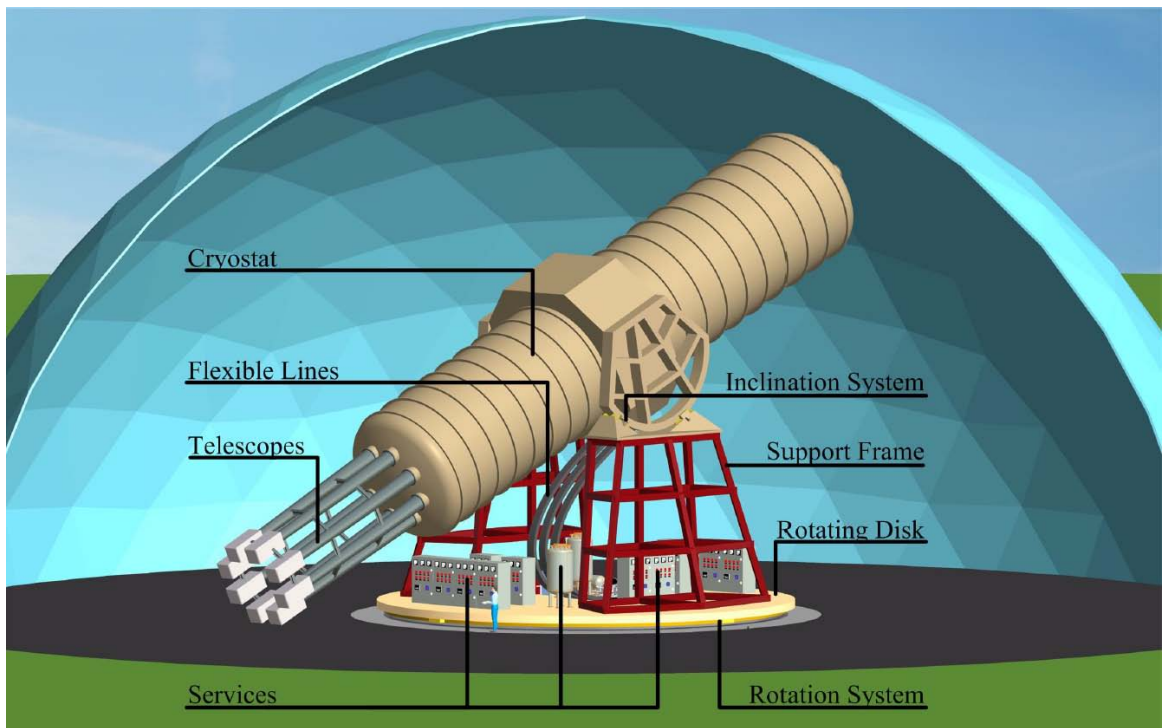
Figure 8.2: Schematic view of the IAXO proposal. The different parts of the magnet, magnet support, and feeds are labeled. Plot taken from [132].
