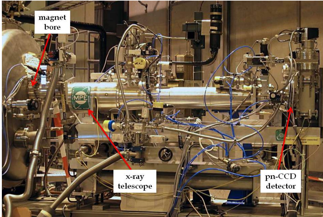
Figure 2.15: The x-ray telescope and the CCD detector system on the CAST experiment.
