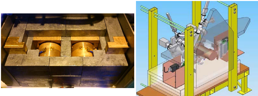
Figure 7.7: Left: Photo of the Sunset shielding partially opened in which the inner copper layer and the external lead are visible. Right: Scheme of the Sunset Micromegas shielding design where the position of the plastic scintillators can be observed.
