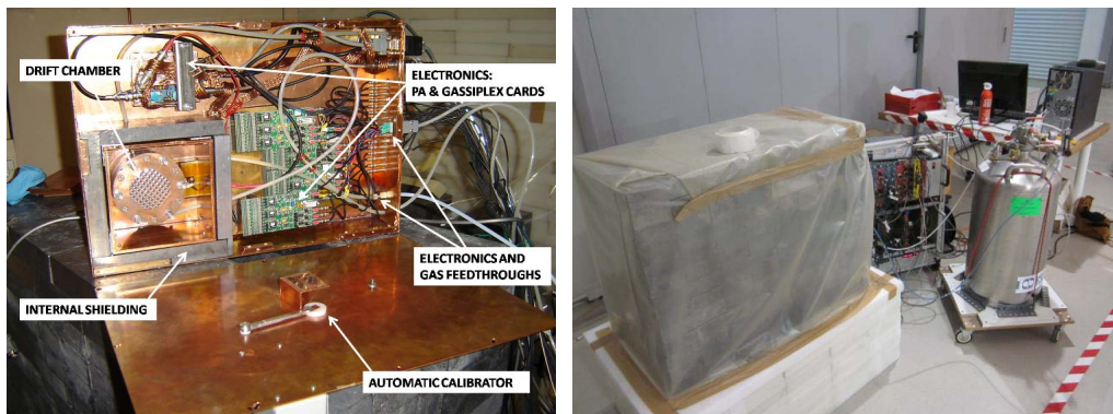
Figure 7.2: Left: CAST Micromegas replica at the LSC, in which the different parts are inside the Faraday cage are labeled. Right: Set-up with 100 mm of external lead, in which the electronics and the dewar used to flush nitrogen are shown.
