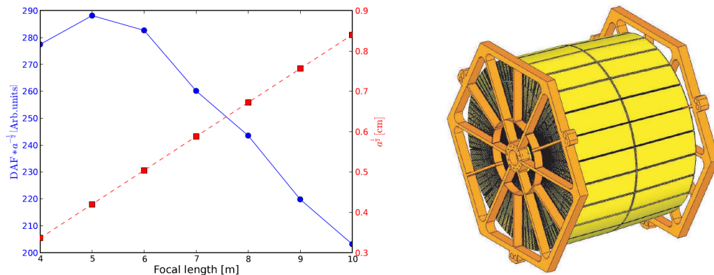
Figure 8.3: Left: Focal length versus spot size \sqrt{a} (red squares) and the throughput of the optics (blue dots) which is calculated by dividing the a quantity related with the efficiency of the optics (DAF) by \sqrt{a} . The optimum is found for f = 5 m. Right: Isomorphic side view of the telescope, in which the "spider-web" structure is shown. Plots taken from [132].
