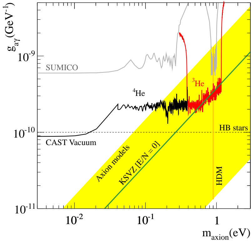
Figure 6.10: Parameter space m_a - g_{a\gamma} excluded by the CAST experiment for the vacuum and {}^4\text{He} phase (black line) and the latest results of the {}^3\text{He} period (red line). The yellow band is the most favored region for the axion models and the green solid line corresponds to the KSVZ model ( E/N = 0 ). Plot taken from [72].
