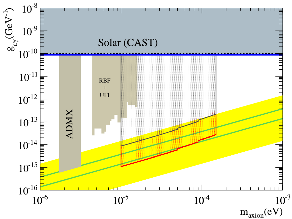
Figure 10.14: Sensitivity regions for long thin microwaves cavities, with a geometry fixed by the desired directional effect. Two different scenarios has been computed: a conservative one (black region) and the optimistic one (red region).
