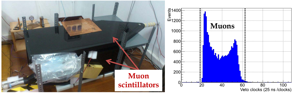
Figure 7.4: Left: Set-up at the Zaragoza lab, both plastic scintillators for the muon rejection are shown. Right: Time difference between the delayed Micromegas trigger and the scintillator. The black dashed lines delimit the region for the rejection of events induced by muons in the off-line analysis. The shape of the distribution is due to the drift velocity in the Micromegas detectors.
