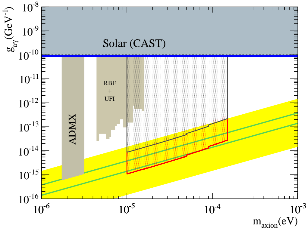
Figure 9.5: Sensitivity regions for the microwaves cavities presented, with a geometry fixed by the desired directional effect. The conservative option (black region) is calculated for Q = 1000 and t_{step} = 30000 s, using the parameters from table 9.1. For the red region more optimistic parameters have been considered with a quality factor of Q = 20000 , t_{step} = 3000 s, and a volume 10 times larger than the previous one. Some excluded regions by haloscopes and CAST are also shown. The yellow band indicates the region favored by the QCD axion models, being the green lines two representative benchmark models, the KSVZ (upper one) and the DSFZ model. Plot taken from [139].
