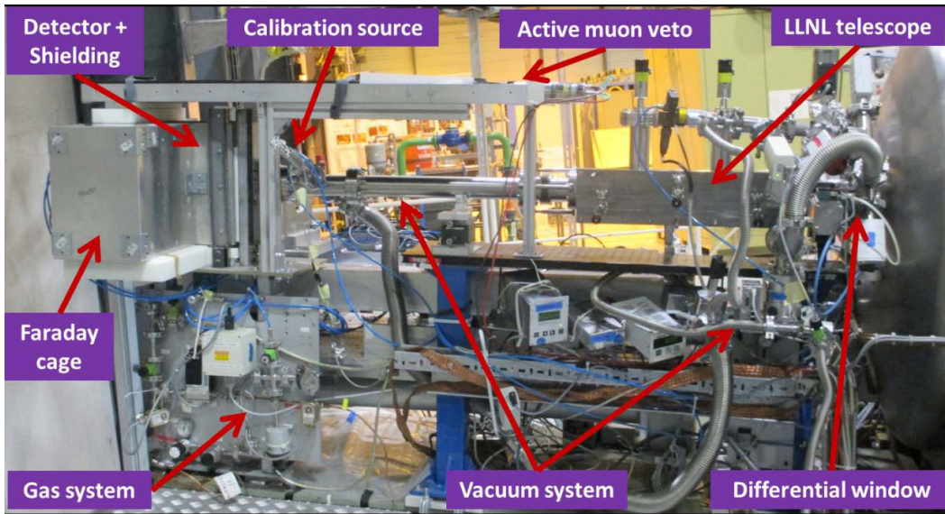
Figure 10.11: Photo of the new Sunrise Micromegas+XRT system in the CAST experiment. The different parts on the set-up are labeled.
