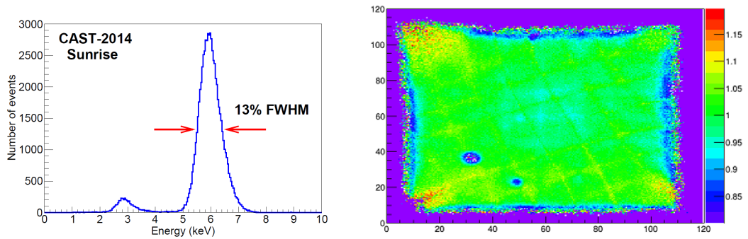
Figure 7.12: Left: ^{55}\text{Fe} calibration spectrum of the Sunrise Micromegas. Right: Gain uniformity of the Sunrise Micromegas. The dead areas (in purple) show lower values than the unity (in green) and lie outside the axion-sensitive area
