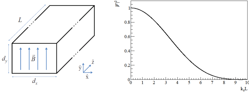
Figure 9.1: Left: Sketch of the cavity geometry used for the calculations. Right: |F|^2 versus k_z L for a single incoming axion momentum k as expressed in equation 9.5. Plots taken from [139].
