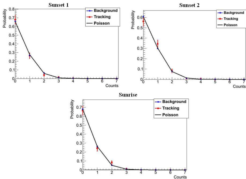
Figure 5.12: Distribution of the number of counts using a time binning of 15 minutes. The distribution has been obtained following the schema from figure 5.11.
