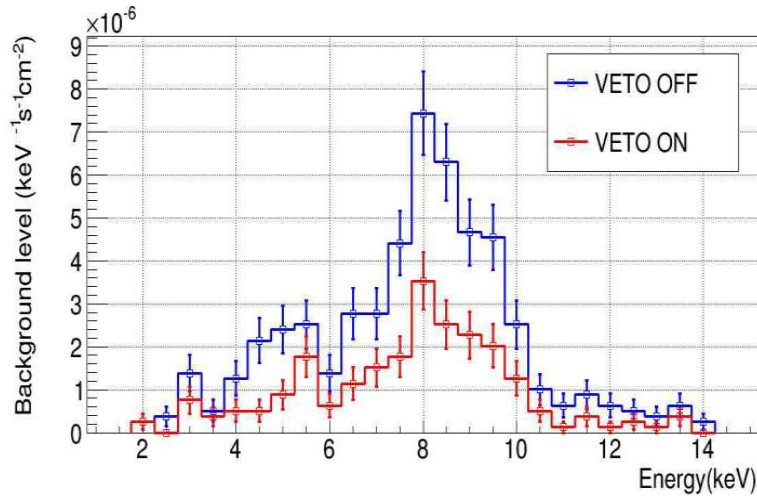
Figure 7.5: Background spectra from the measurements performed in the Zaragoza lab by using the muon scintillator. The blue line corresponds to the level before the muon subtraction, while the red line is the final level after the veto cut.
