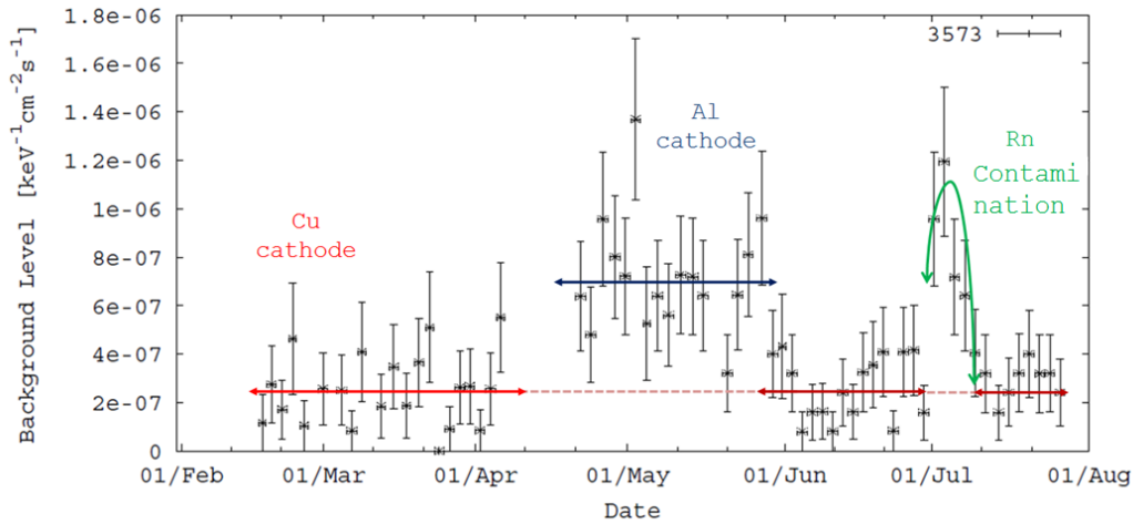
Figure 7.3: Background level in the LSC during 2011. An the ultra-low background level (red arrows) was interrupted due to the measurements of the aluminum cathode (blue arrow) and the ^{222}\text{Rn} intrusion (green arrow). Plot taken from [120].
