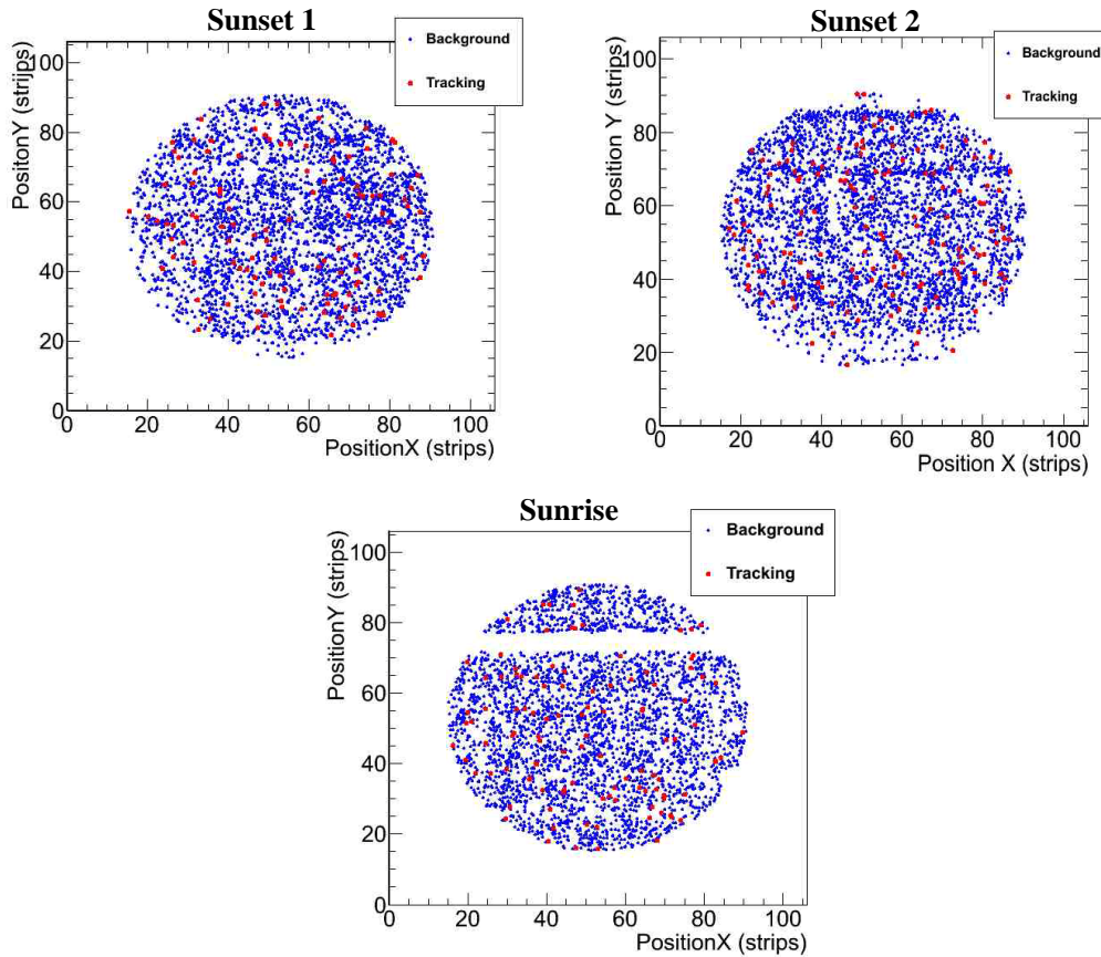
Figure 5.10: Spatial distribution of the background (blue dots) and tracking (red dots) events during the 2011 data taking campaign in the Micromegas detectors. Only the events inside the coldbore area and in the RoI ( [2 - 7] keV) are represented.
