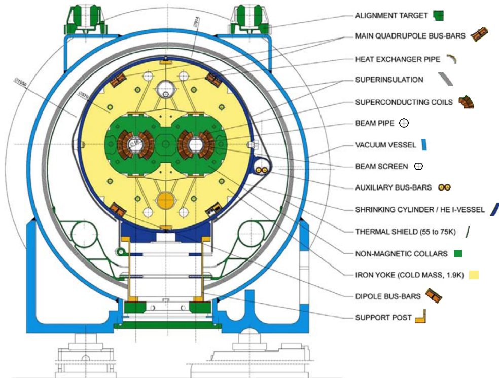
Figure 2.3: Standard cross section of a LHC dipole magnet.
