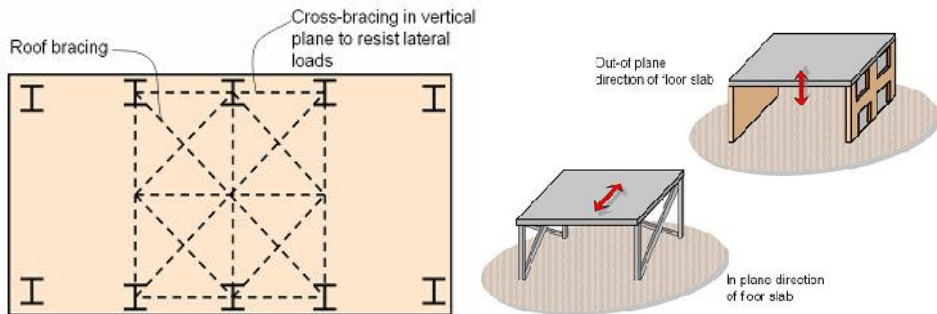
Figure 6. Floor Diaphragm Source: Szakats, Gregory A.J, 2006
