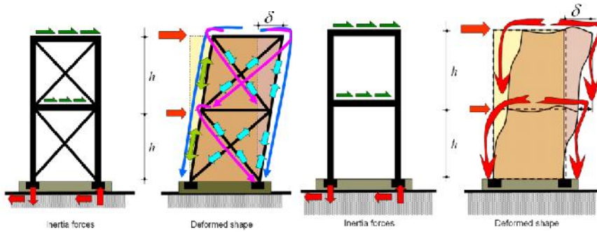
Figure 4. Bracing to Retain a Building. Source: Szakats, Gregory A.J, 2006
