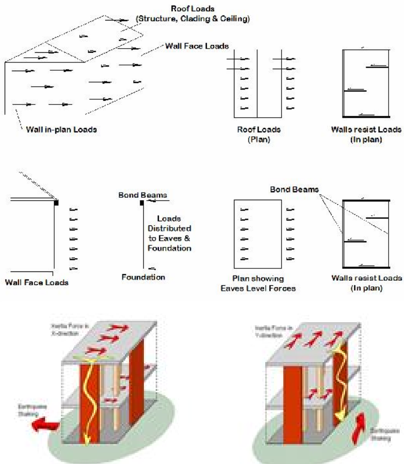
Figure 3. Chronology of Horizontal Force on Building Source: Szakats, Gregory A.J, 2006
