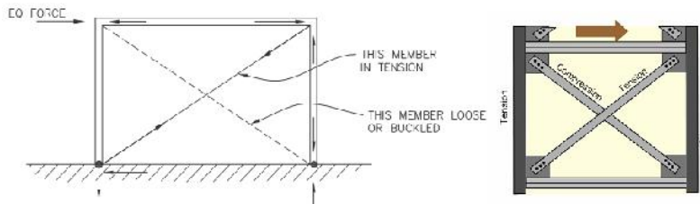
Figure 5. Framework as Tension Retaining Source: Szakats, Gregory A.J, 2006
