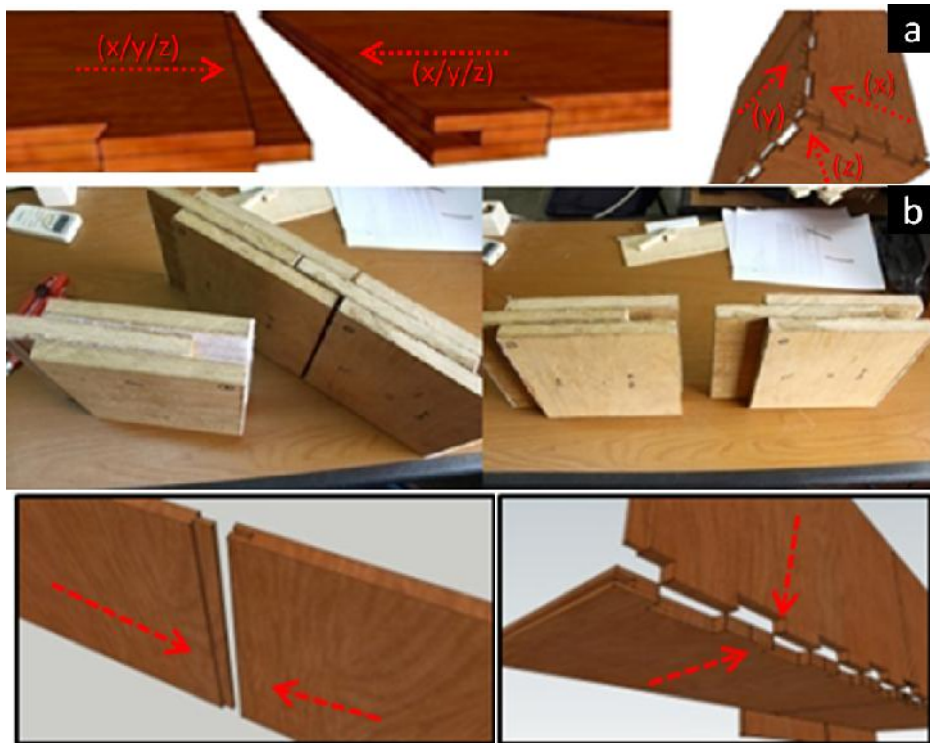
Figure 14. G-Feet Sticky House Details: a) Joints between the Straight Plane and the Angled Plane, b) G-feet's Joints Mock-up (scale 1:1) Source: author's documentation
