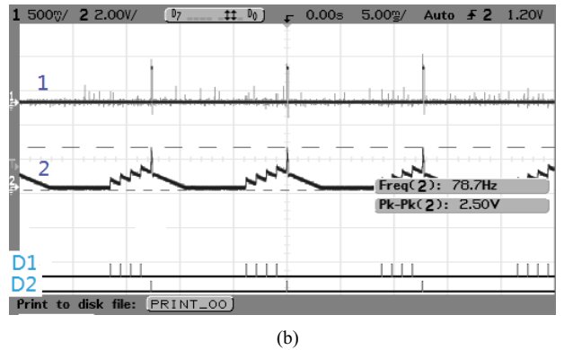
Fig. 17. (a) Time cost of MATLAB simulation from the input to the output is linear. (b) Snapshot of neuron response of the SC chip. D1 and D2 are the input spikes for digital block. Signal 1 and 2 are recorded from analog IF neuron output. During recording, the time scale is 5 ms/div. The time delay between spike input and the resultant output is less than 1 ms.
