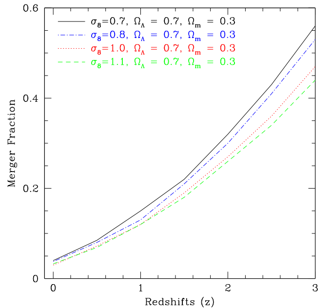
Figure 3. The evolution of the halo merger fraction for haloes with M_{\text{halo}} > 10^{12} M_{\odot} as a function of the value of \sigma_8 . The range we show here is for \sigma_8 = 0.7 –1.1, with the highest halo merger fractions for those evolving within a universe that has the lowest \sigma_8 .
