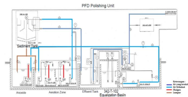
Gambar 1. PFD Polishing Unit.
