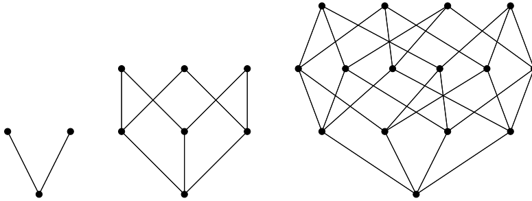
Figure 1: The first three truncated hypercubes T_2 , T_3 , and T_4
