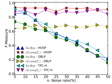
(c) Varying n\%
