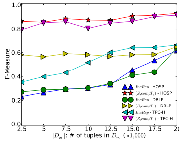
(b) Varying |D_m|
