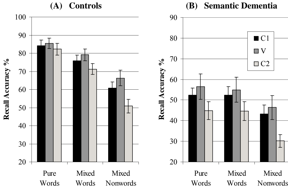
Figure 6: Recall of Phonemes by Syllabic Position
