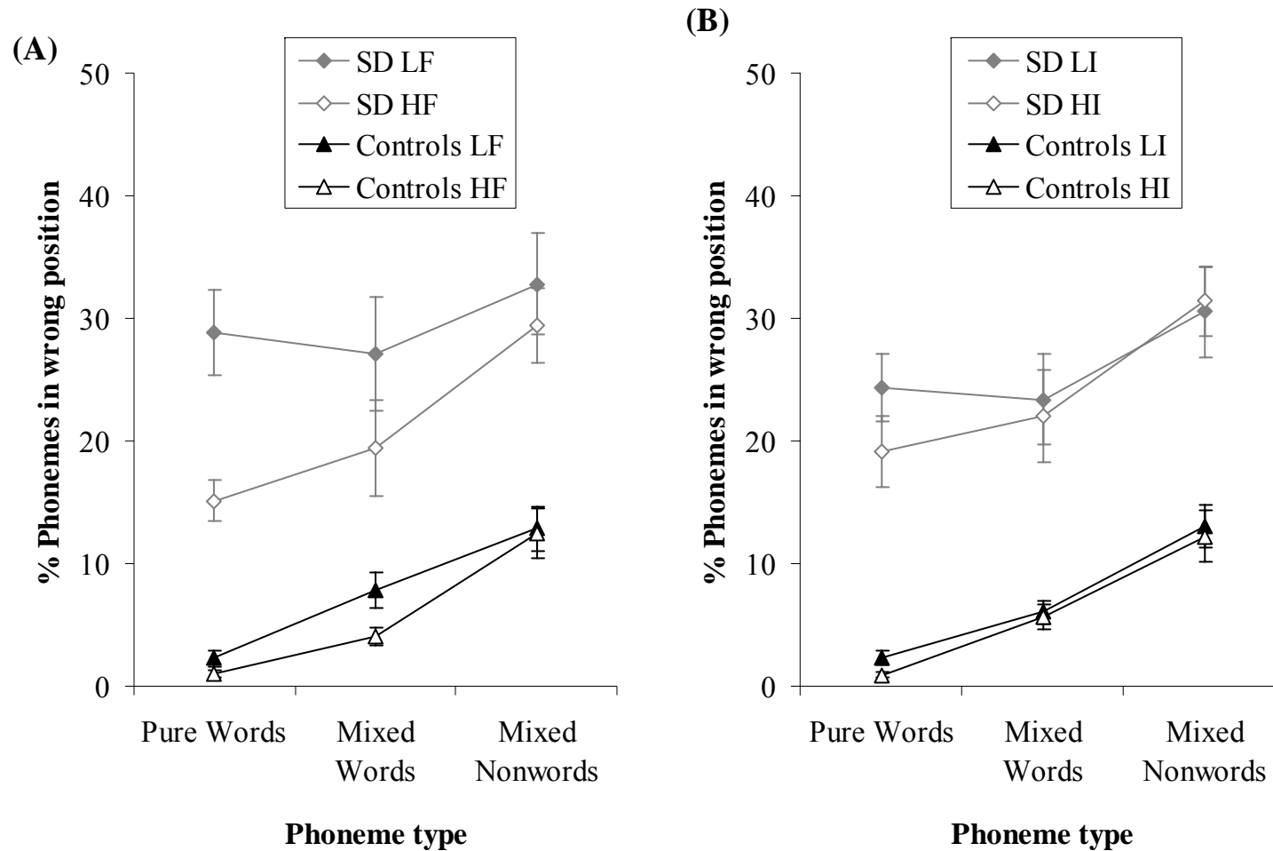
Figure 4: Rate of Phoneme Migrations
