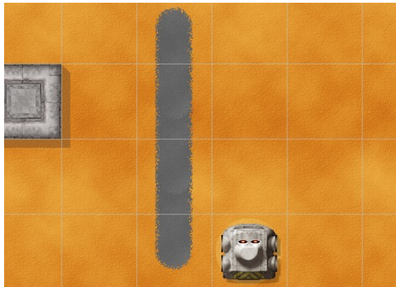
Figure 4. Copyline Problem
