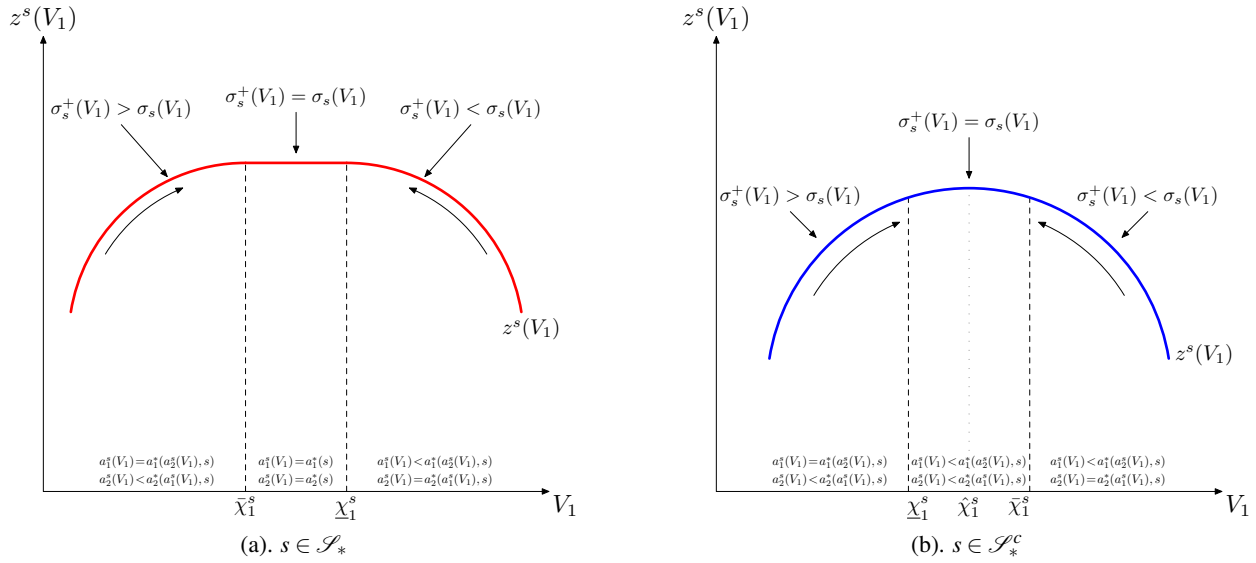
FIGURE 1: Surplus Function z^s(V_1)
