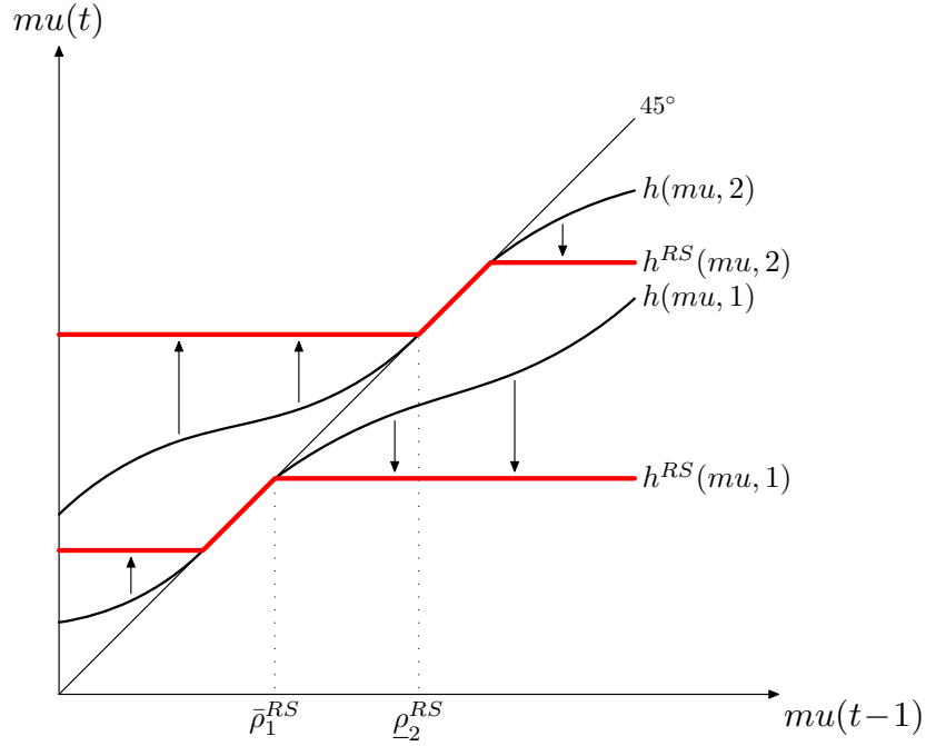
FIGURE 2: Convergence to Pure Risk-Sharing
