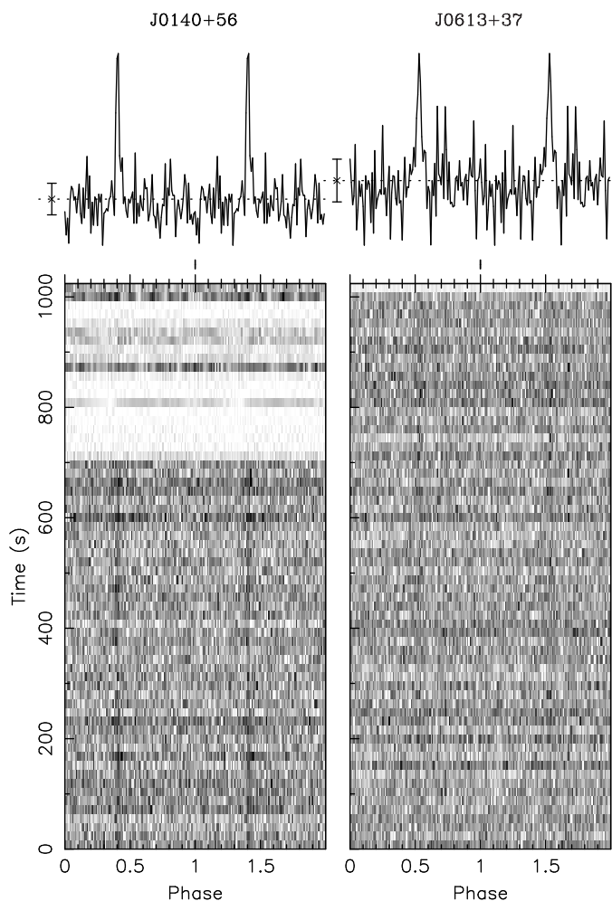
Fig. 7. Discovery plots of PSRs J0140+5622 (left) and J0613+3731 (right). The bottom panels shows the signal strength as a function of time and rotational phase. Some RFI is masked, showing up as white-outs. The top panels shows the folded profiles, repeated twice for clarity.
