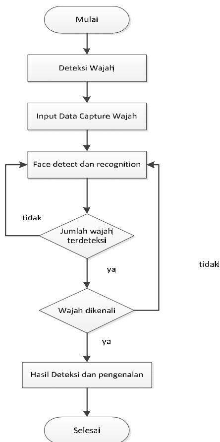
Gambar 3. Flowchart Image Processing
