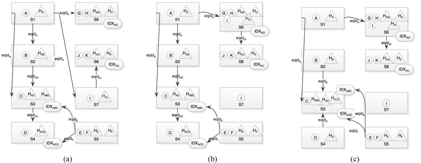
Fig. 6. Example of minimizing eqid shipment (base hash tables used only locally are omitted). (a) No replication. (b) With replication. (c) Minimum eqid shipment.
