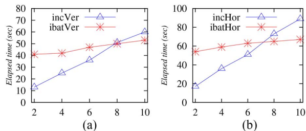
Fig. 11. Experimental results for refined batch algorithms. (a) Ver, |\Delta D| : *1M tuples. (b) Hor, |\Delta D| : *1M tuples.
