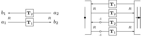
Figure 5: Left: MD unit element, with shifts T_1 and T_2 . Right: Series/parallel connection of two MD unit elements, one with sign inversion.
