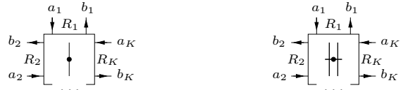
Figure 4: Left: Series K -port adaptor (scattering junction). Right: Parallel K -port adaptor.
