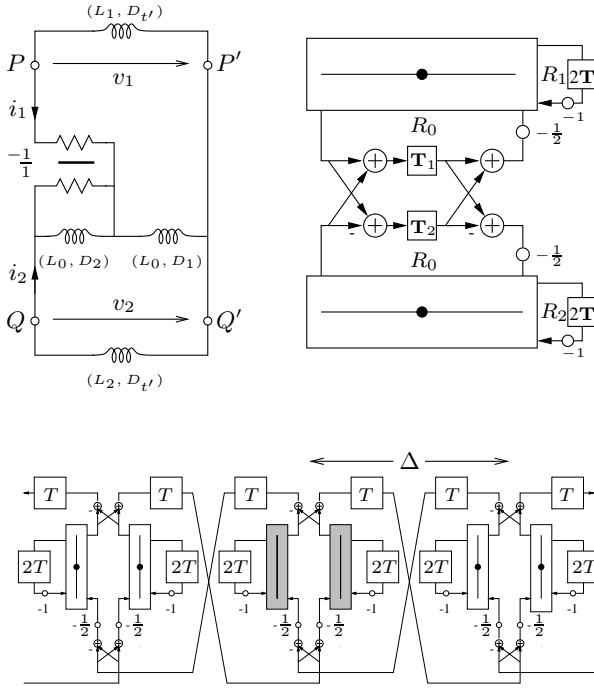
Figure 6: Top left: MDKC for the (1+1)D transmission line system (21), with L_1 = v_0 l - r_0 , L_2 = v_0 r_0^2 c - r_0 , and L_0 = r_0 / \sqrt{2} . Top right: MDWD network, with R_1 = 2L_1/T' , R_2 = 2L_2/T' and R_0 = 4L_0/T_1 , where we have used the step sizes of (4), as well as T' = 2\Delta (see comment at end of Section 2.5). Bottom: Expanded signal-flow diagram (port-resistances not shown). Grey/white coloration of junctions indicates that calculations are to be performed at alternating time instants.
