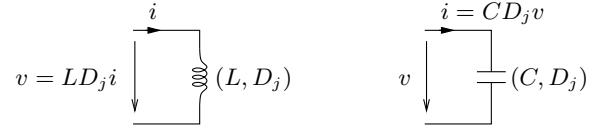
Figure 1: Left: Inductor of inductance L , and direction t_j . Right: Capacitor of capacitance C and direction t_j .
