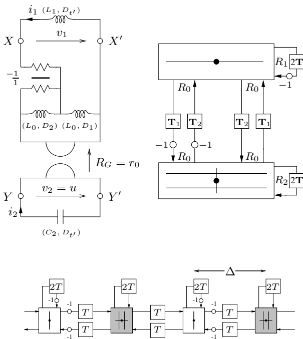
Figure 7: Top left: Transformed MDKC for the (1+1)D transmission line system (21), with L_1 = 2\Delta(v_0l - r_0) , C_2 = 2\Delta(v_0c - 1/r_0) , and L_0 = \sqrt{2}\Delta r_0 . Top right: MDWD network, with R_1 = 2L_1/T' , R_2 = T'/(2C_2) and R_0 = r_0 . Bottom: Expanded signal-flow diagram (port-resistances not shown). Grey/white coloration of junctions indicates calculation at alternating time instants.
