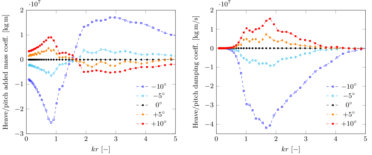
Figure 12: Inclination effects on the modified Dutch Tri-floater’s heave-pitch coupling added mass and wave damping.
