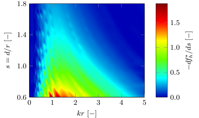
Figure 8: Vertical wave load sensitivity to submergence for a column with heave plate.
