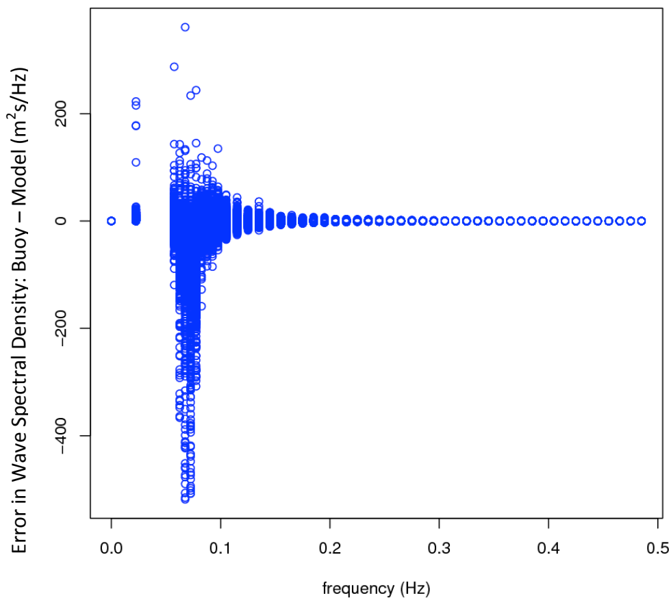
Figure 6: The error between buoy and model of specific energy summed over direction ( \text{m}^2\text{s}/\text{Hz} ) for each frequency and each time record plotted against frequency (Hz)
