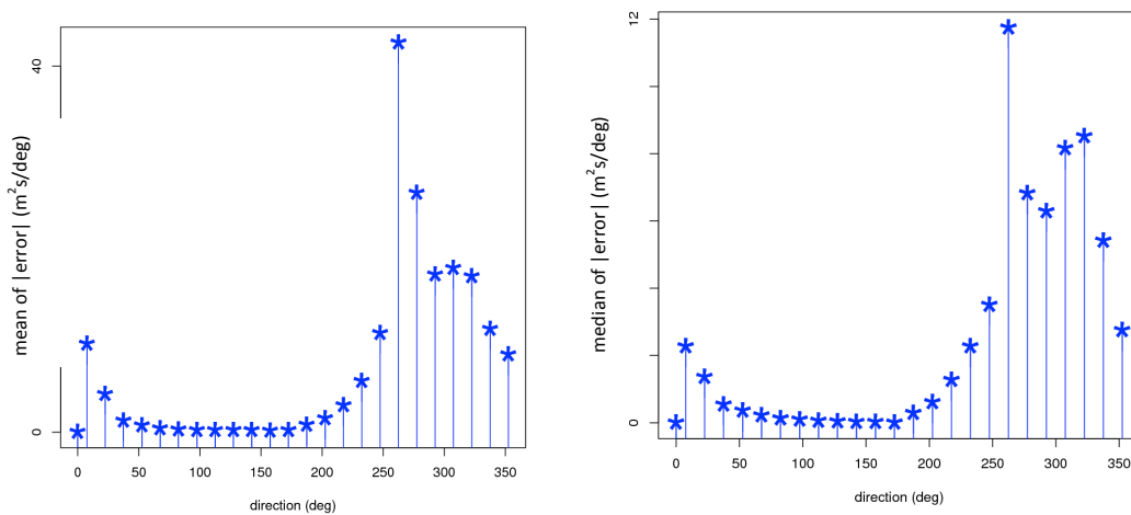
Figure 5: The mean (left) and median (right) of the errors of specific energy summed over frequency ( \text{m}^2\text{s}/\text{deg} ) within each directional bin against direction
