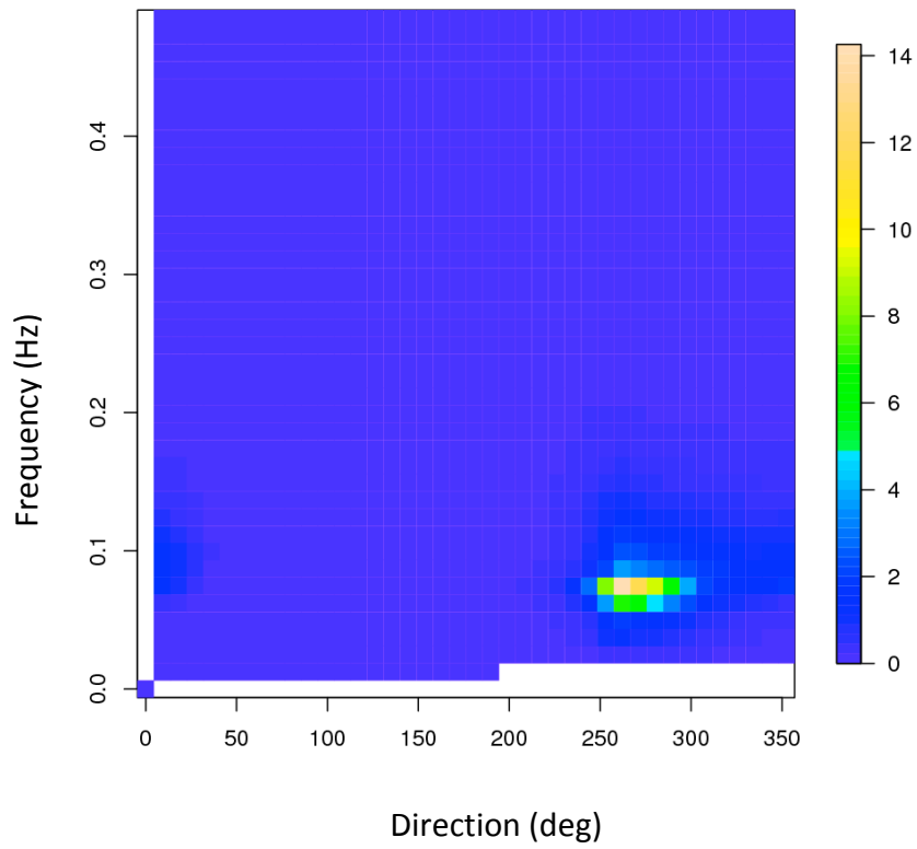
Figure 8: x-axis: direction (deg); y-axis: frequency (Hz); colour scale: mean of the absolute value of error between buoy and model within each (re-binned) spectral bin ( \text{m}^2\text{s}/\text{Hz-deg} ) [27, 28]
