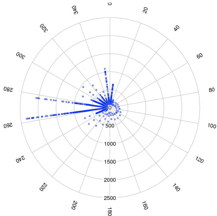
Figure 4: The absolute value of the error between buoy and model of specific energy summed over frequency ( \text{m}^2\text{s}/\text{deg} ) for each direction and each time record plotted against direction (degree) [26]
