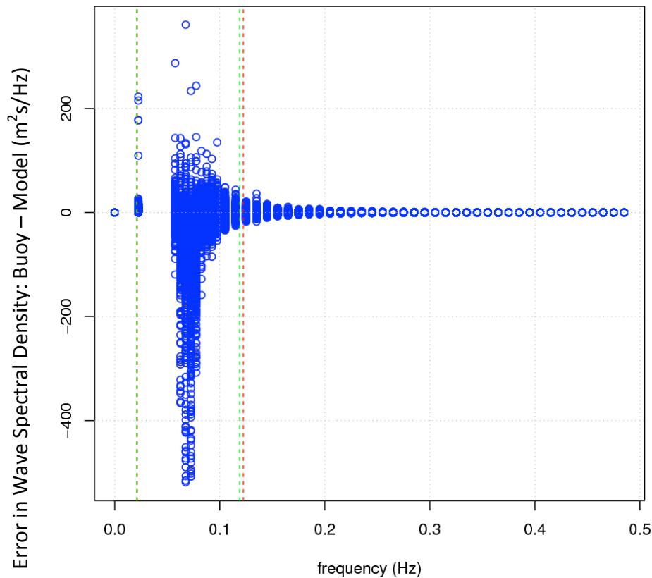
Figure 10: The error between buoy and model of specific energy summed over direction ( \text{m}^2\text{s}/\text{Hz} ) for each frequency and each time record plotted against frequency (Hz) with lines representing cut-off frequencies at which waves switch from shallow to intermediate (left lines) and intermediate to deep (right lines) for buoy (red) and model (green)
