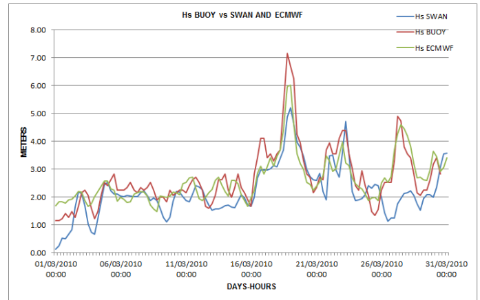
FIGURE 3: Comparison of H_s acquired by the buoy, ECMWF and SWAN.
