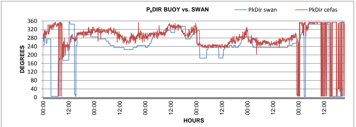
FIGURE 11: Peak wave direction between buoy and SWAN in degrees
