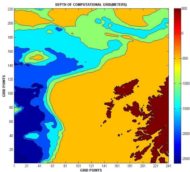
FIGURE 1: depth of computational grid in meters
