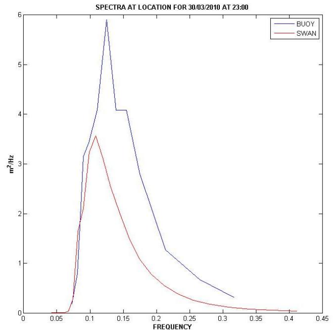
FIGURE 4: 1D wave spectra compared
