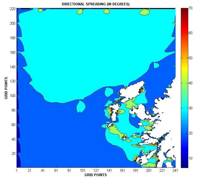
FIGURE 8: Directional at last timestep in degrees
