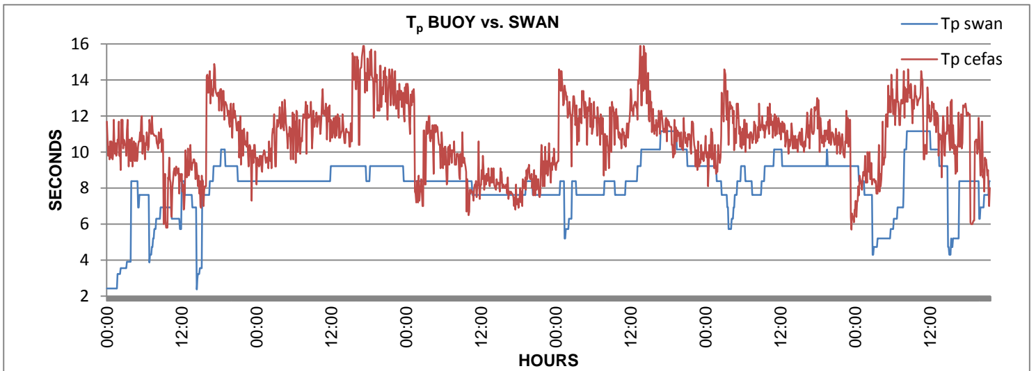
FIGURE 10: Peak period of buoy and SWAN, in seconds
