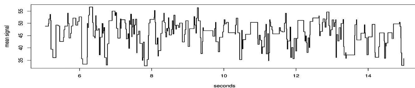
Figure 1 An example output from the plot.squiggle function. Plotted are the events data extracted from a single read. The y-axis is the mean electronic signal reported for the pore, and the x-axis is time in seconds.
