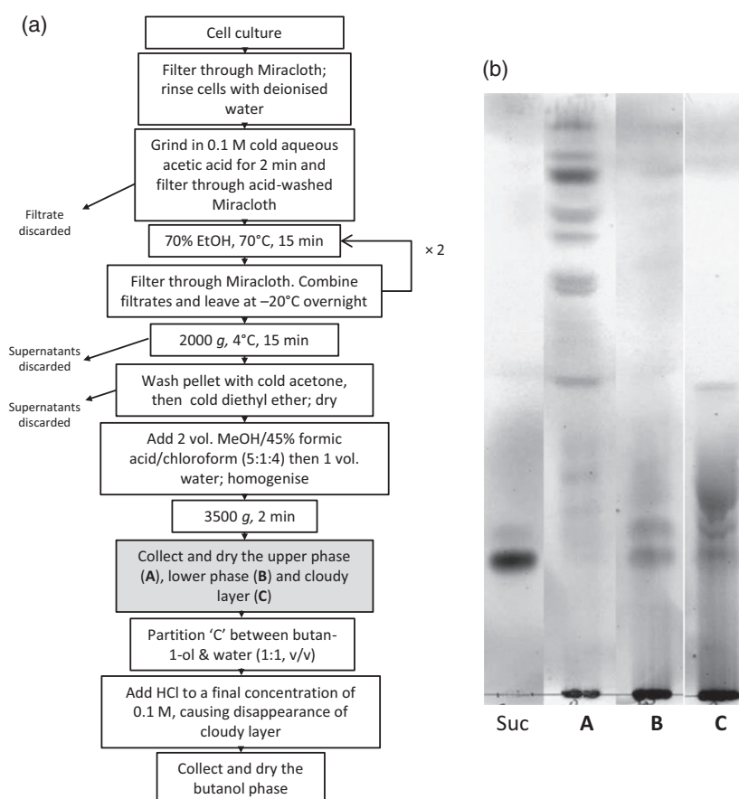
Figure 3. Purification of glycosylinositol phosphorylceramide (GIPC) from Rosa cell culture. (a) GIPC purification scheme adapted from Buré et al. (2011). (b) Thin-layer chromatography (TLC) of the phase A, B and C obtained during the step shaded grey in (a). Suc, sucrose marker.
