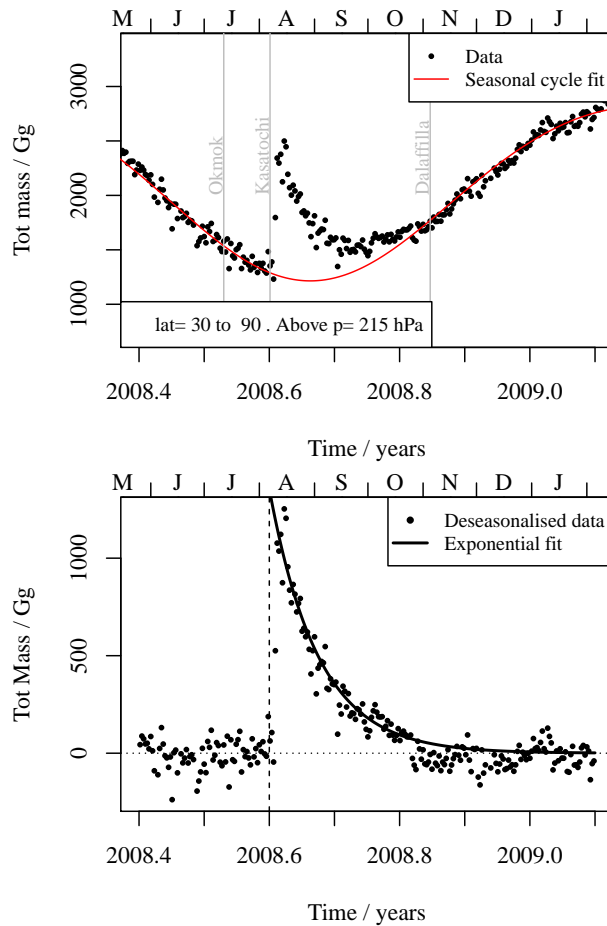
Figure 11. Isolating the volcanic \text{SO}_2 from the background value (with its spurious seasonal cycle). The example shown is for the eruption of Kasatochi.
