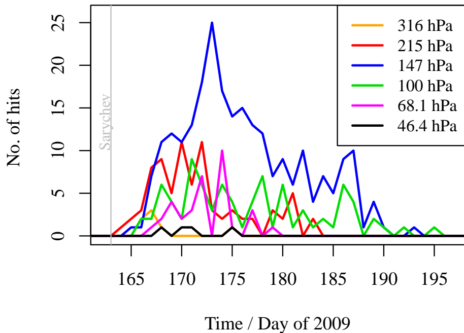
Figure 5. Number of observations of volcanic SO 2 in the days following the eruption of Sarychev. An observation is defined in the same way as in Fig. 3 and Table 1. The eruption is marked as occurring on day 163 (12 June 2009).
