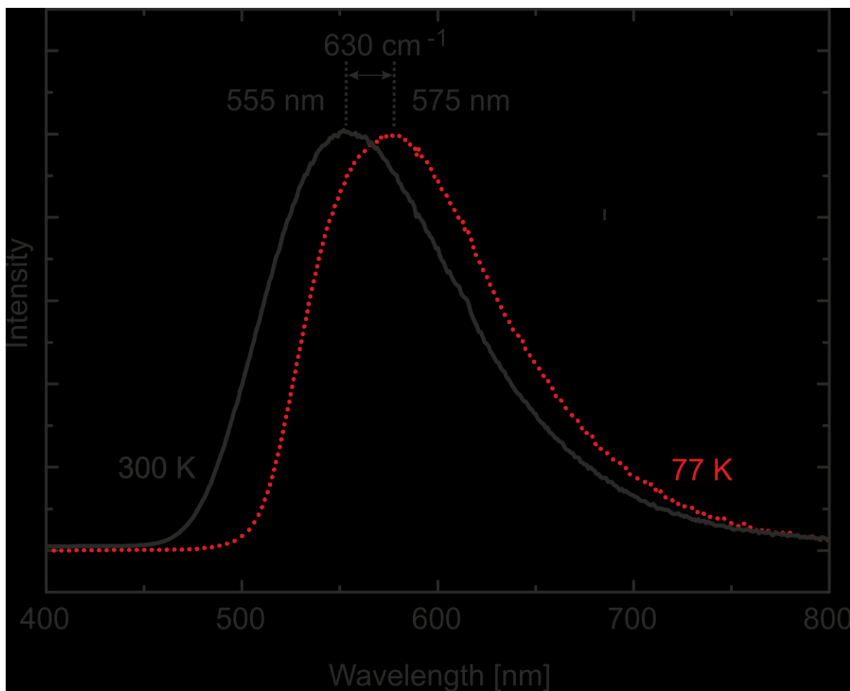
Figure 2: Emission spectra of compound [Cu(POP)(tmbpy)][BF 4 ] ( 2 ) (powder) recorded at temperatures of 300 K and 77 K. The samples were excited at \lambda_{\text{exc}} = 350 nm.
