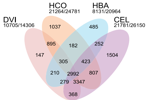
Figure 2. Comparison of the Dictyocaulus viviparus proteome to that of other rhabditid nematodes. Venn diagram illustrating the orthoMCL clustering of the predicted proteome of Dictyocaulus viviparus (DVI) to those of Caenorhabditis elegans (CEL), Heterorhabditis bacteriophora (HBA) and Haemonchus contortus (HCO). The numbers of proteins clustered and the total number of predicted proteins is given below each species' name.
