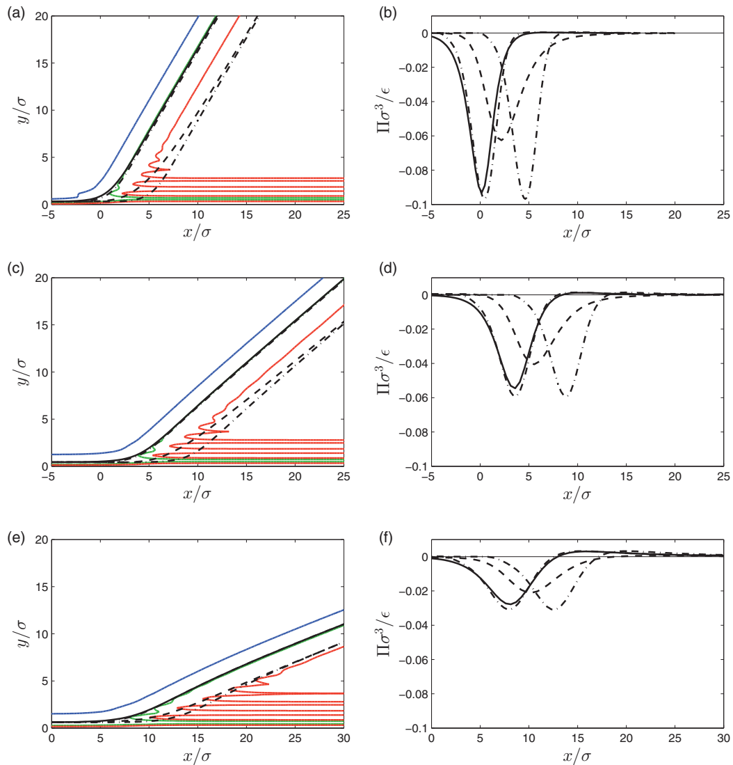
FIG. 7. Density contours (left column, (a), (c), and (e)) and disjoining pressures (right column, (b), (d), and (f)) for three contact line regions. The top, middle, and bottom rows depict results for the three different substrate strengths \alpha_w \sigma^3 / \epsilon = \{1.25, 1.375, 1.47\} , corresponding to Young contact angles 60.0^\circ , 41.1^\circ , and 20.4^\circ , respectively. In the left column, the contour lines correspond to number densities (n - n_{\text{vap}}) / (n_{\text{liq}} - n_{\text{vap}}) = \{0.05, 0.5, 0.95\} from left to right, respectively. Height profiles h_{\text{II}} and h_{\text{III}} as in (29) and (31) are represented by the dashed and solid lines, respectively. h_{\text{I}} as defined by (27) is plotted with dashed-dotted lines twice, to match h_{\text{II}} and h_{\text{III}} for large film thicknesses, through a corresponding choice of h_B in (28). We note that in the left column, the solid, one of the dashed-dotted lines, and the density isoline representing (n - n_{\text{vap}}) / (n_{\text{liq}} - n_{\text{vap}}) = 0.5 are virtually indistinguishable. The right column depicts the disjoining pressure profiles. The dashed line represents \Pi_{\text{II}}(x) as defined in Eq. (26), the dashed-dotted line represents \Pi_{\text{I}}(h_{\text{I}}(x)) for the two shifted cases h_{\text{I}} as depicted in the left column, and employing data of the adsorption isotherm for the disjoining pressure, using (20). For comparison with Eq. (12), the scaled curvature -\gamma_{\text{vd}} \left( h'_{\text{III}} / \sqrt{1 + (h'_{\text{III}})^2} \right) / dx is plotted with the solid line.
