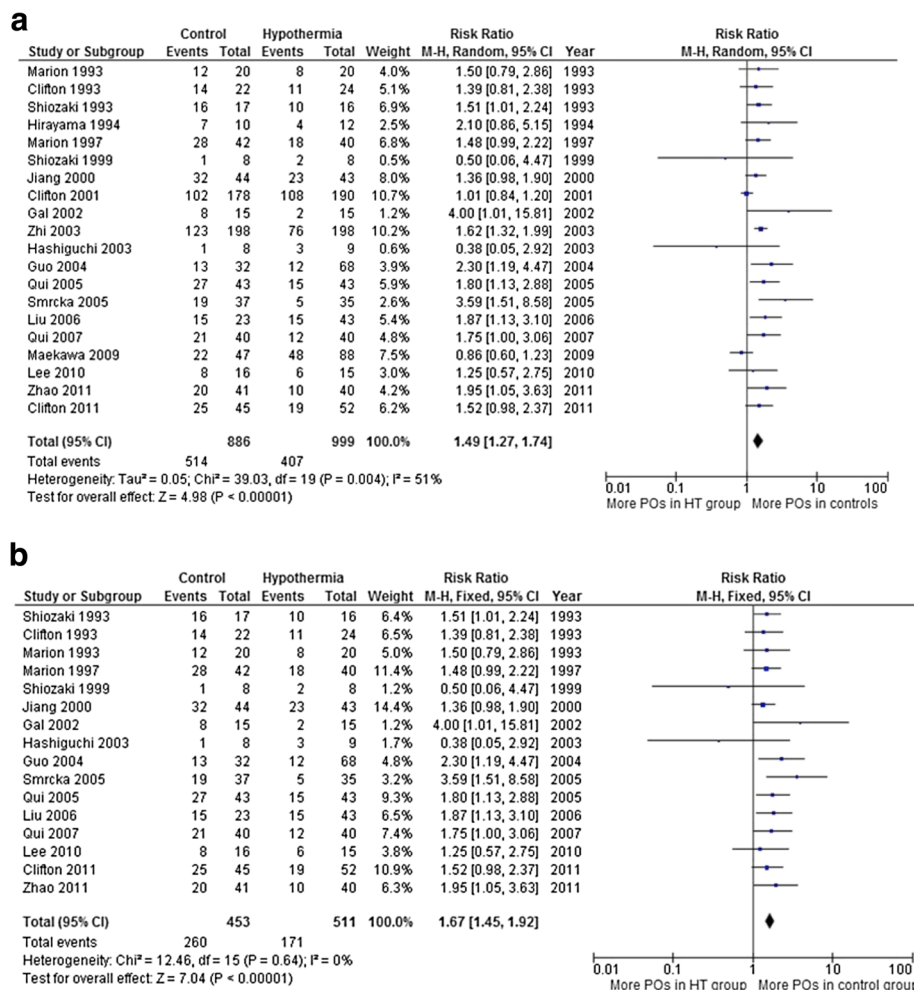
Figure 2 Poor outcome at final follow-up. (a) In total 20 trials involving 1,885 patients reported death, vegetative state, and long-term disability. When the results of 20 randomised controlled trials (RCTs) that evaluated poor outcome were statistically aggregated, therapeutic hypothermia was associated with a significant reduction in poor outcome (relative risk (RR) = 1.49, 95% CI = 1.27, 1.74, P < 0.00001 ). (b) Trials assessed as lower risk of bias: 16 trials, involving 964 patients, and assessed as lower risk of bias (domain-based assessment) were included in this analysis. When the results of 16 RCTs that evaluated poor outcome were statistically aggregated, therapeutic hypothermia was associated with a significant reduction in poor outcome (RR = 1.67, 95% CI = 1.45, 1.92, P < 0.00001 ).
