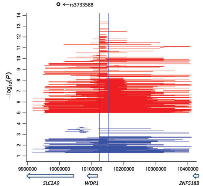
Figure 2. Local interactions in the 4p16.1 region (red) and those remaining significant ( P_{\text{int}} < 0.05 ) in conditional tests on the lead SNP rs3733588 (blue) in ARIC. Each horizontal line represents an interaction between two SNPs at the start and end locations; two vertical lines mark the 30-kb window described in the main text; y-axis: interaction P -values in the -\log_{10} scale; x-axis: genomic location in base pair (UCSC hg19/NCBI 37.3); arrow bar showing transcription direction and location of the gene ( italic ) below the bar.
