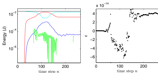
Figure 5: Left: energy partition for the system of parameters as given in the caption to Figure 4, as a function of time step n . Linear string energy \mathfrak{h}_L (red), nonlinear string energy \mathfrak{h}_K (blue), string/barrier collision energy \mathfrak{h}_c (green), finger energy \mathfrak{h}_f (cyan) and total energy \mathfrak{h} (black). Right: normalized energy variation \epsilon = (\mathfrak{h}^{n+1/2} - \mathfrak{h}^{1/2})/\mathfrak{h}^{1/2} .
