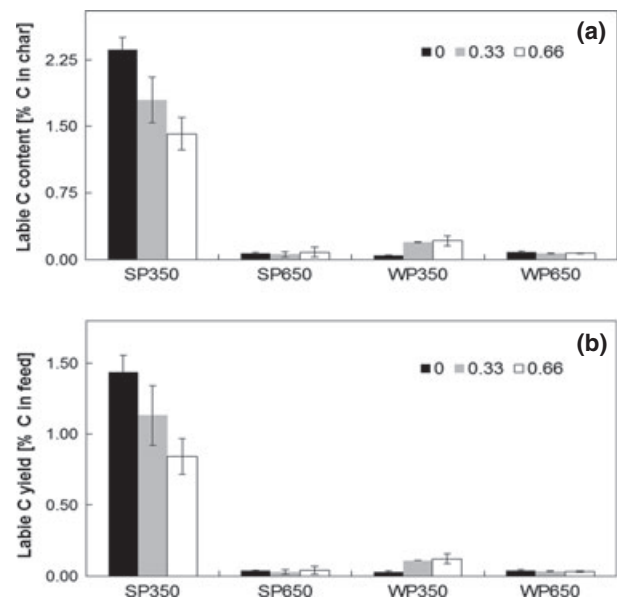
Fig. 5 Labile-C content of SP and WP biochar expressed on (a) char carbon basis, (b) feedstock carbon basis.
