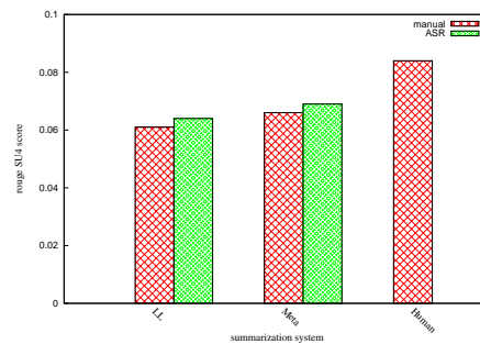
Fig. 7. ROUGE-SU4 Scores
