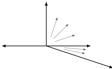
FIGURE 5. A schematic picture of the fan in the proof of Lemma 24
