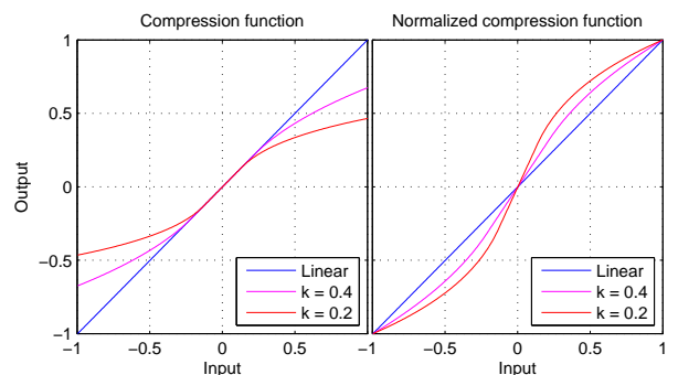
Figure 2: Illustration of the compression function without (left) and with signal normalization (right).
