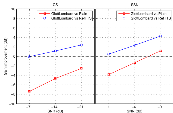
Figure 5: Improvement in gain (dB) for the proposed system (GlottLombard) in comparison to original speech (Plain) and reference TTS system (RefTTS) in competing speech (CS) and speech-shaped noise (SSN) with three different SNRs.
