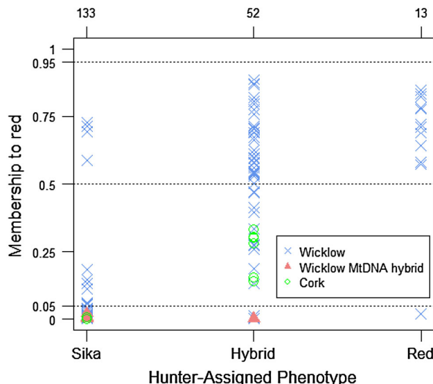
Fig. 4 The estimated proportion of ancestry ( Q ) for all animals from Co. Wicklow and Co. Cork ( n = 198 ) plotted against their hunter-assigned phenotype. Mitochondrial hybrids, which are beyond the detection of the nuclear markers, were only found in Wicklow and are represented by triangles. 13 animals from Wicklow were excluded as they did not have a phenotype assigned
