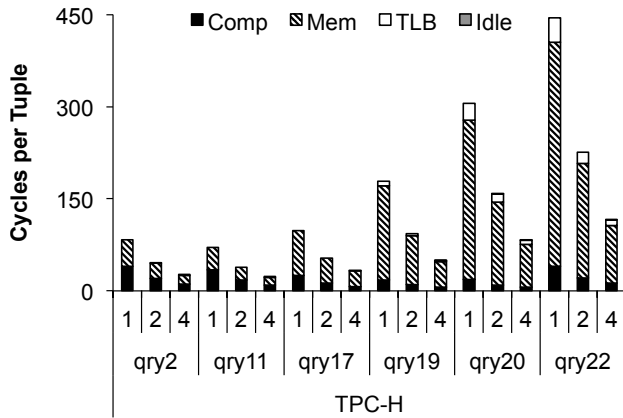
(a) Widx walkers cycle breakdown for TPC-H queries
