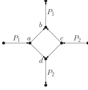
Figure 3: The digraph D .
