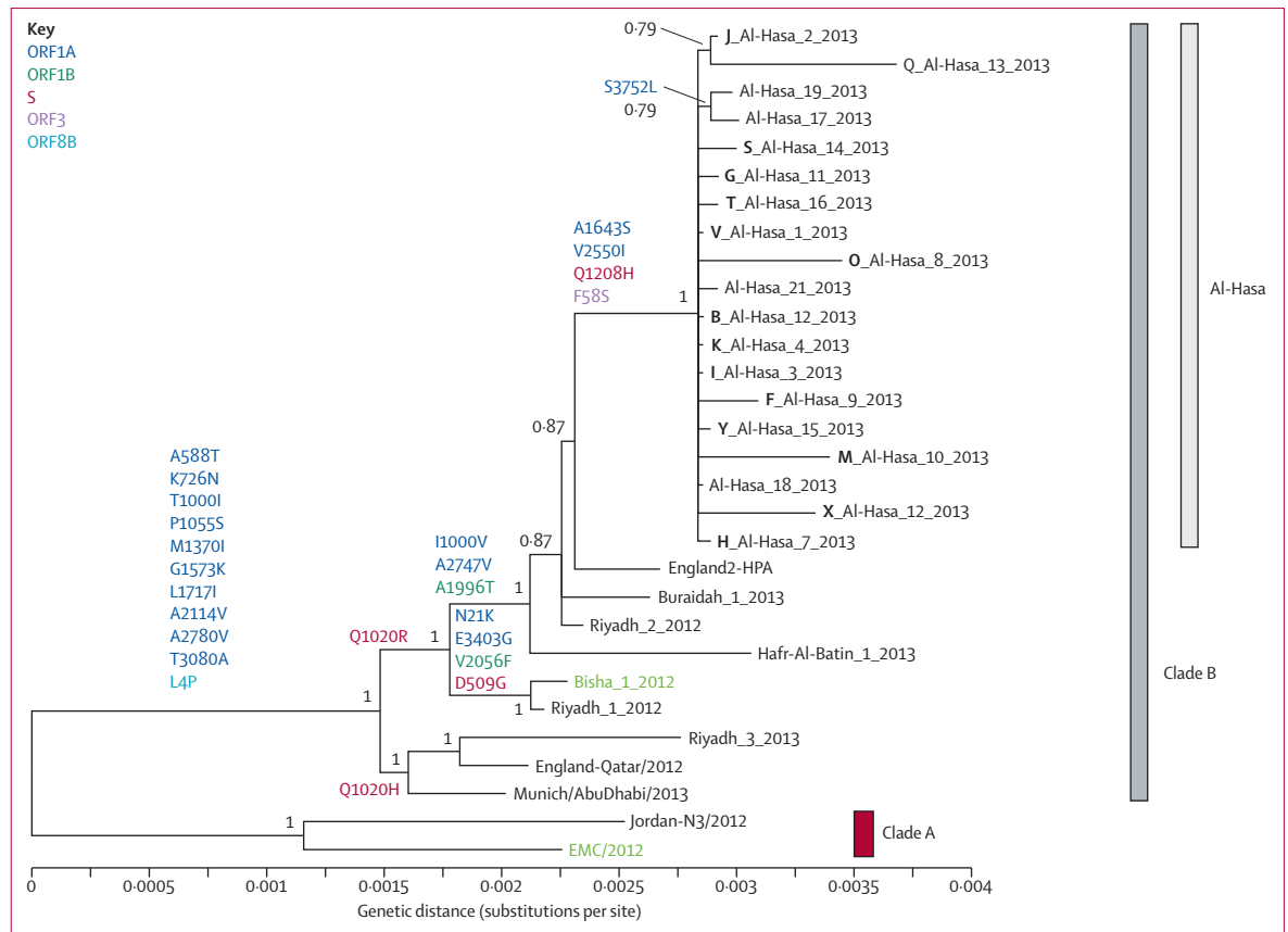
Figure 2: Bayesian-inferred phylogeny of all 21 new sequences Combined with the published genomes (EMC/2012 [GenBank number JX869059], Jordan-N3 [KC776174], Munich/AbuDhabi [KF192507], England-Qatar_2012 [KC667074], Al-Hasa_1_2013 [KF186567], Al-Hasa_2_2013 [KF186566], Al-Hasa_3_2013 [KF186565], Al-Hasa_4_2013 [KF186564], and England2-HPA [no number available]). The single letter patient codes from Assiri and colleagues 16 are given where appropriate. Clade A, clade B, and the Al-Hasa cluster are marked with vertical bars. Aminoacid changes along the internal branches were established through likelihood-based ancestral state reconstruction. These are shown above the branches and colour-coded by ORF. The scale bar below the phylogeny shows the genetic distance, in substitutions per site, from the arbitrary midpoint root. Bayesian posterior probabilities for each clade are given above the relevant node. MERS-CoV=Middle East respiratory syndrome coronavirus. ORF=open reading frame.
