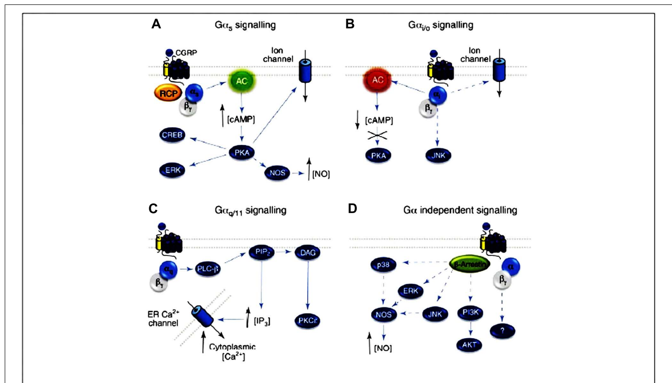
FIGURE 3 | CGRP receptor-mediated intracellular signaling. (A) G s signaling increases AC (green) activity, elevating intracellular cAMP, activating PKA and subsequently many potential downstream effectors. (B) The CGRP receptor might also couple to G i/o , reducing AC (red) activity, decreasing intracellular cAMP and reducing PKA activity. (C) CGRP signaling via G q activates PLC- \beta , which cleaves PIP 2 into IP 3 and DAG, resulting in elevated intracellular Ca 2+ and PKC activation. (D) The CGRP receptor might also utilize G \alpha -independent signaling, and G \beta\gamma - or b-arrestin-mediated signaling
