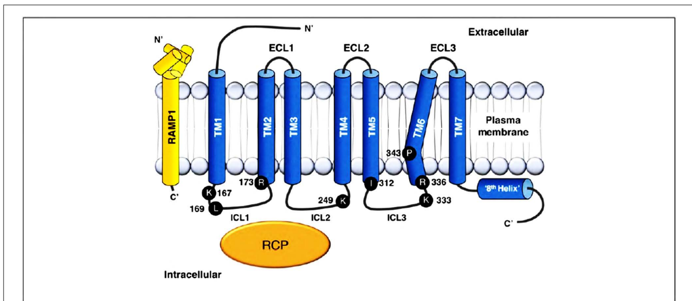
FIGURE 2 | Structure of CGRP receptor. CGRP receptor components and important residues for receptor signaling and internalization. The CGRP receptor is formed by CLR (blue), RAMP1 (yellow), and RCP (orange). Functionally important residues are shown as single letter abbreviations.
