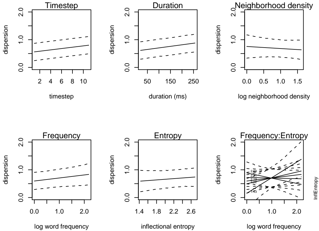
Figure 1: Partial effects of the numeric predictors for vowel dispersion. Dotted lines show MCMC-based 95% highest posterior density (HPD) intervals based on 100,000 samples.
