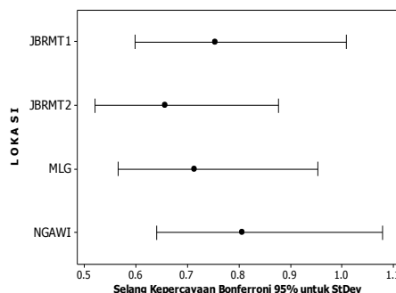
Gambar 3 Plot uji Bartlett
