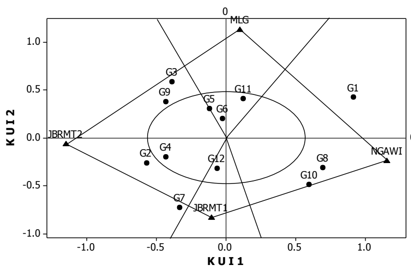
Gambar 5 Biplot AMMI2
