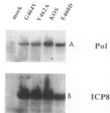
FIG. 4. Western blot analysis of mock-infected and virus-infected cell extracts. Each lane contained approximately 50 \mu g of total protein. Filters were probed successively with polyclonal sera directed against HSV Pol (A) and ICP8 (B). The viruses used are indicated above the lanes.
