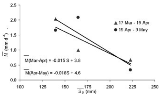
Fig. 6. Association between landscape-class melt rate and average pre-melt SWE in complex tundra landscapes, Granger sub-catchment ( <5\text{ km}^2 ), 1999. The two linear relationships between pre-melt SWE and melt rate shown are similar enough that coefficients and constants could be averaged.
