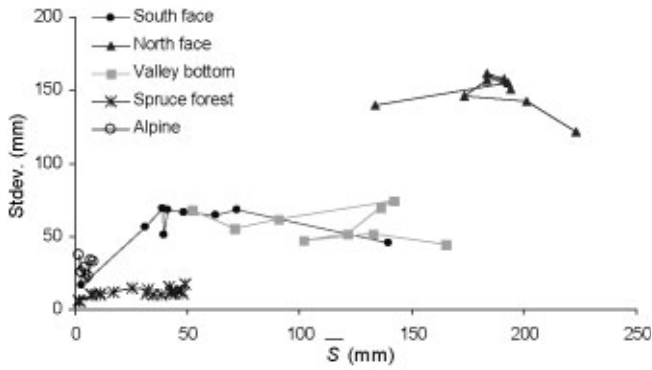
Fig. 4. Change in standard deviation with \bar{S} during melt, Granger-complex tundra (north face, south face, valley bottom), boreal-forest and alpine-tundra landscape classes, 1999.
