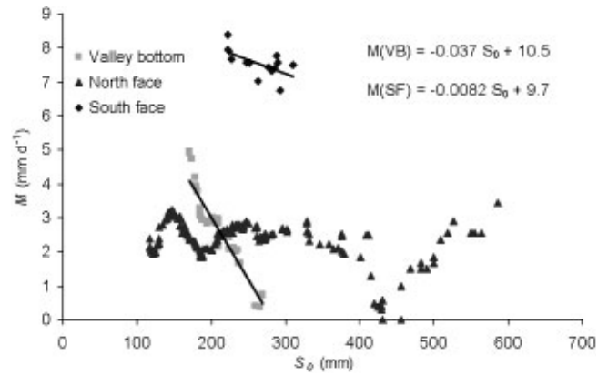
Fig. 5. Association between melt rate and average pre-melt SWE, 19 April–16 May 1999, for valley bottom, south face and north-facing 20° tundra slopes, Granger sub-catchment. Best-fit linear relationships shown where a trend is evident.
