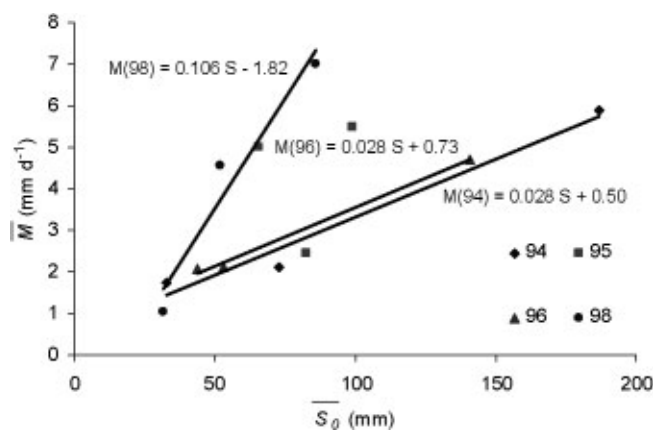
Fig. 7. Association between landscape-class melt rate and average pre-melt SWE for varied landscape classes, Wolf Creek catchment ( 185\text{ km}^2 ), 1994–98. Linear relationships are shown where they were evident. The years 1994 and 1996 have sufficiently similar trends that the coefficients and constants could be averaged.
