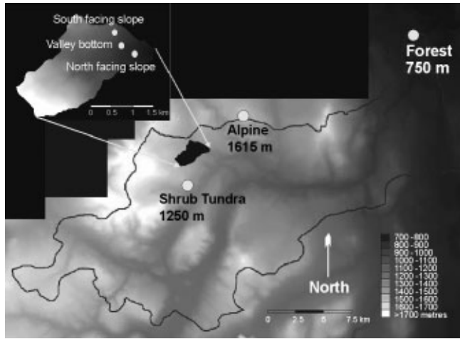
Fig. 1. Digital elevation map of Wolf Creek catchment, with regular snow-survey locations (Buckbrush = shrub tundra) and Granger sub-catchment marked. The Granger sub-catchment is magnified to show location of snow-survey transect and slopes.
