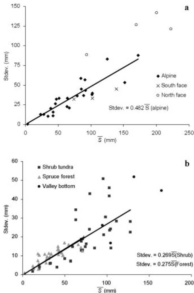
Fig. 3. Winter (December–April) average SWE, \bar{S} , and standard deviation for landscape-class-based snow surveys, 1993–99. (a) Windswept landscape classes including alpine tundra, and the complex 20^\circ north- and south-face tundra slopes in Granger sub-catchment. Linear relationship between standard deviation and \bar{S} is shown for the alpine landscape class only. (b) Sheltered landscape classes including shrub tundra, valley bottom tundra (Granger) and boreal-forest sites. Linear relationships between standard deviation and \bar{S} are shown for the shrub tundra and boreal-forest landscape classes only.
