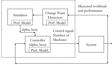
Figure 1: Architectural diagram of the control framework.
