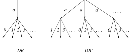
Figure 8: An example of two infinite databases with \text{appr}(DB) \subseteq \text{appr}(DB') but DB \not\subseteq DB' . Here DB' is not label-finite.
