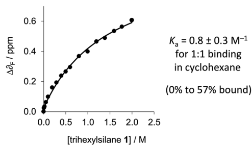
Fig. 5 1 : 1 binding data for the titration of trihexylsilane (1) against a constant concentration of perfluoro- tert -butanol (2) (1 mM in cyclohexane at 298 K). Additional data are presented in the ESI. †
